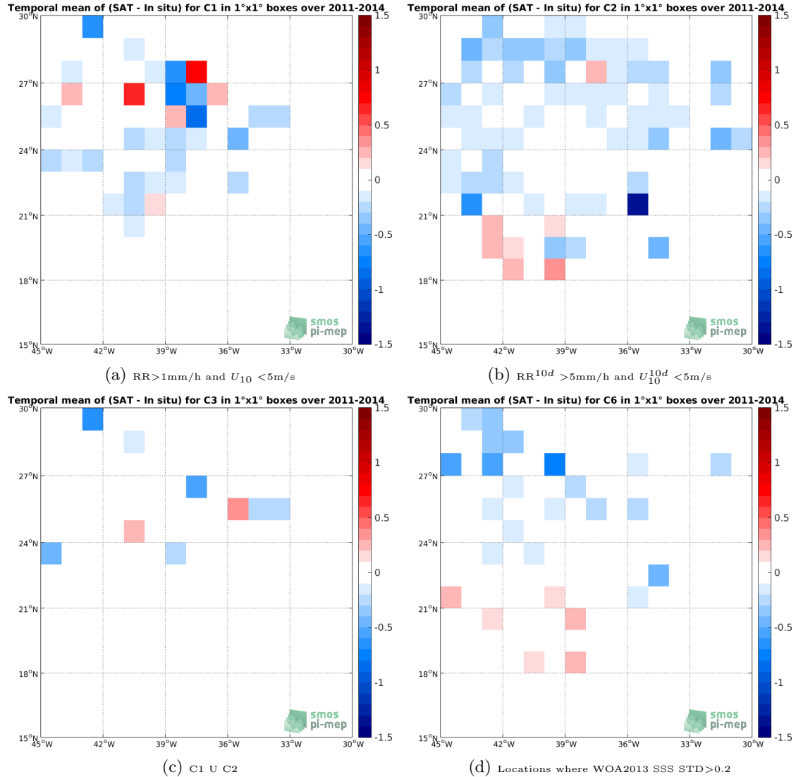
Figure 11: Temporal mean gridded over spatial boxes of size 1^\circ \times 1^\circ of \Delta SSS (SMOS-L3-CATDS-CECOS-IFREMER-V2-1DAY-0.5DEG - Surface drifters) for 4 different subdatasets corresponding to: RR > 1\text{mm/h} and U_{10} < 5\text{m/s} (a), RR^{10d} > 5\text{mm/h} and U_{10}^{10d} < 5\text{m/s} (b), C1 U C2 (c), Locations where WOA2013 SSS STD > 0.2 (d).
