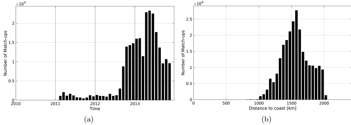
Figure 1: Number of match-ups between Surface drifters and SMOS-L3-CATDS-CECOS-IFREMER-V2-1DAY-0.5DEG SSS as a function of time (a) and as function of the distance to coast (b) over the SPURS 1 Pi-MEP region and for the full satellite product period.
