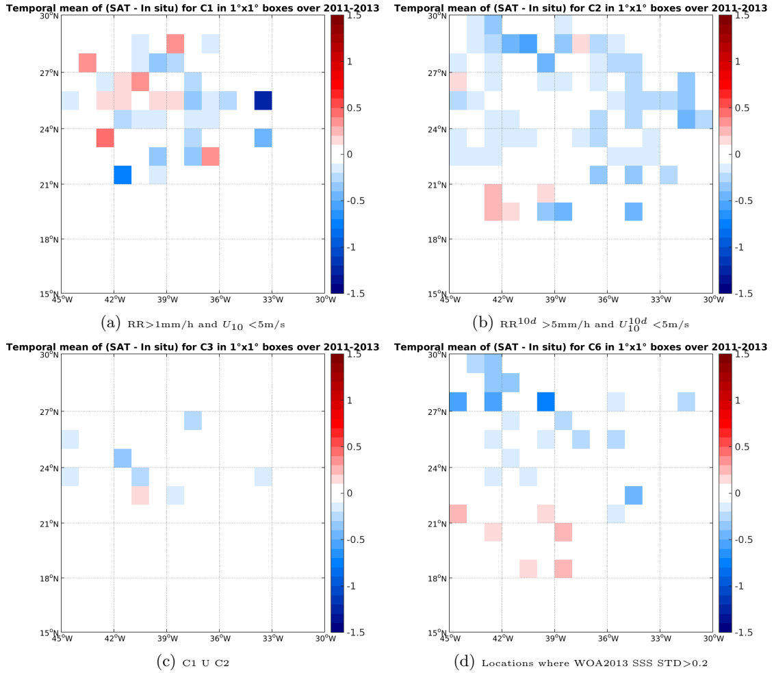
Figure 11: Temporal mean gridded over spatial boxes of size 1°x1° of \Delta SSS (SMOS-L3-CATDS-CECOS-IFREMER-V2-1DAY-0.5DEG - Surface drifters) for 4 different subdatasets corresponding to:RR>1mm/h and U_{10} < 5 m/s (a), RR^{10d} > 5 mm/h and U_{10}^{10d} < 5 m/s (b), C1 U C2 (c),Locations where WOA2013 SSS STD>0.2 (d).
