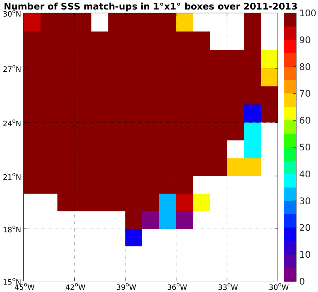
Figure 3: Number of SSS match-ups between Surface drifters SSS and the SMOS-L3-CATDS-CECOS-IFREMER-V2-1DAY-0.5DEG SSS product for the SPURS 1 Pi-MEP region over 1°x1° boxes and for the full satellite product period.
