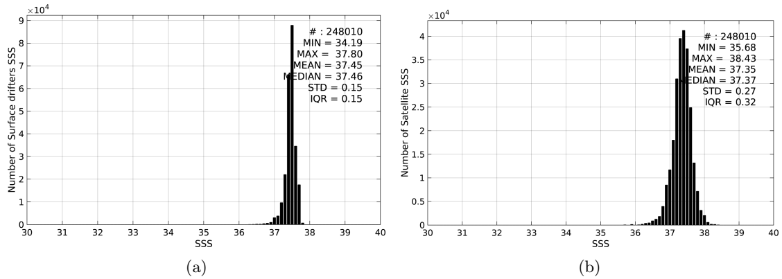
Figure 2: Histograms of SSS from Surface drifters (a) and SMOS-L3-CATDS-CECOS-IFREMER-V2-1DAY-0.5DEG (b) considering all match-up pairs per bins of 0.1 over the SPURS 1 Pi-MEP region and for the full satellite product period.
