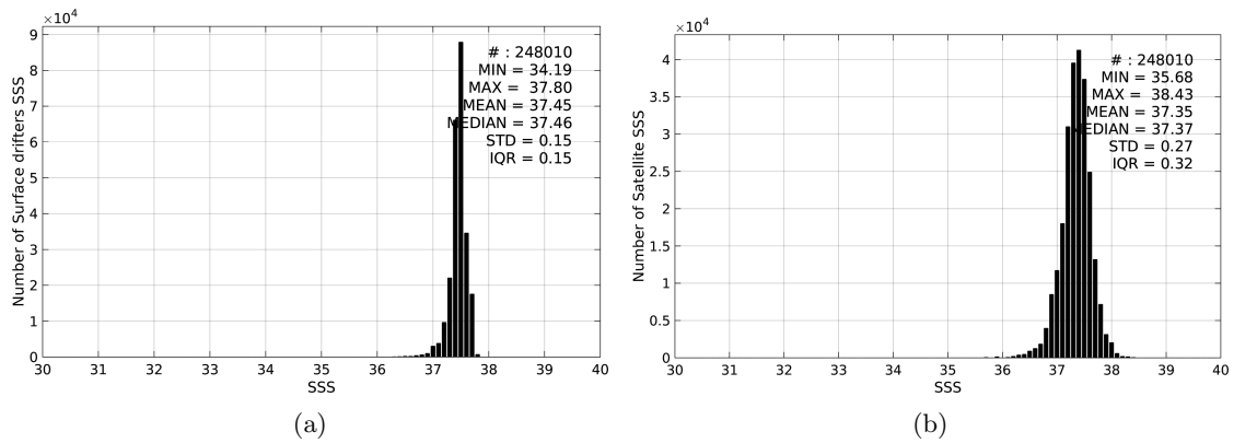
Figure 2: Histograms of SSS from Surface drifters (a) and SMOS-L3-CATDS-CECOS-IFREMER-V2-1DAY-0.5deg (b) considering all match-up pairs per bins of 0.1 over the SPURS 1 Pi-MEP region and for the full satellite product period.
