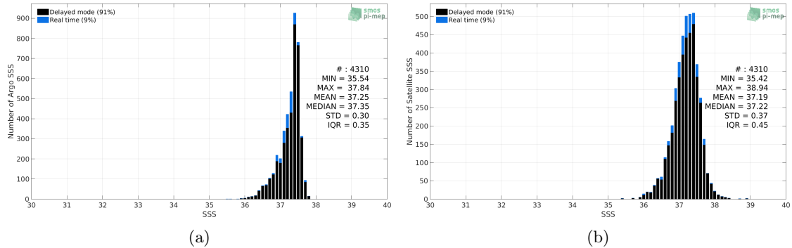
Figure 2: Histograms of SSS from Argo (a) and SMOS SSS L3 v2 - Daily - 0.5 Deg (CATDS-CECOS-IFREMER) (b) considering all match-up pairs per bins of 0.1 over the SPURS 1 Pi-MEP region and for the full satellite product period.
