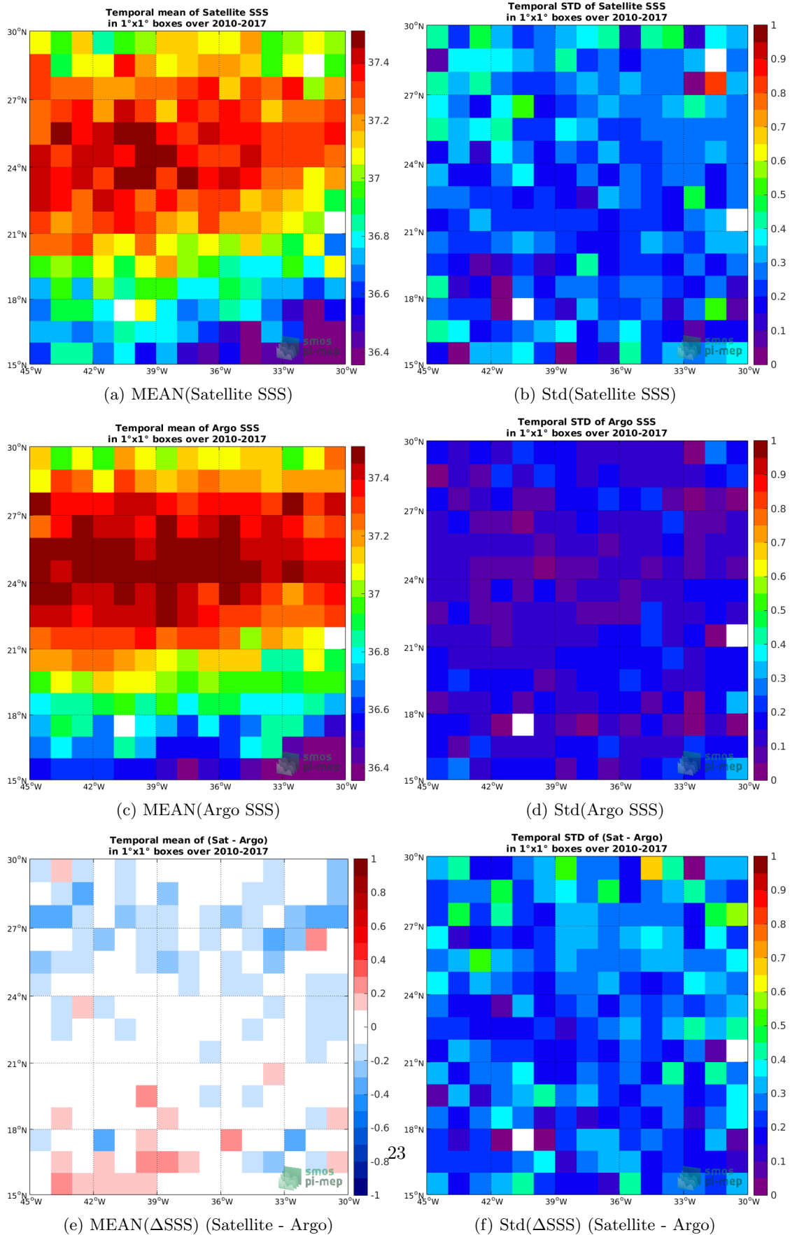
Figure 6: Temporal mean (left) and Std (right) of SSS from SMOS SSS L3 v2 - Daily - 0.5 Deg (CATDS-CECOS-IFREMER) (top), Argo (middle), and of \Delta SSS (Satellite - Argo). Only match-up pairs are used to generate these maps.
