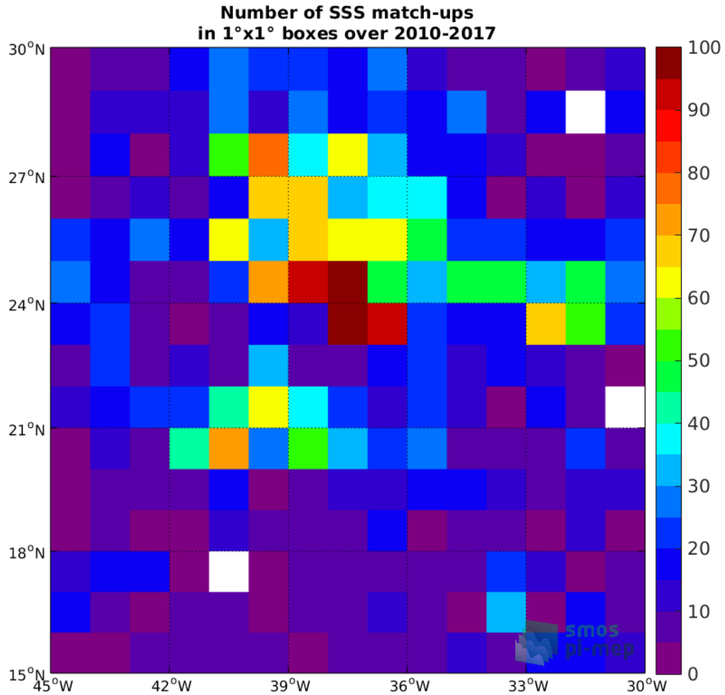
Figure 4: Number of SSS match-ups between Argo SSS and the SMOS SSS L3 v2 - Daily - 0.5 Deg (CATDS-CECOS-IFREMER) SSS product for the SPURS 1 Pi-MEP region over 1°x1° boxes and for the full satellite product period.
