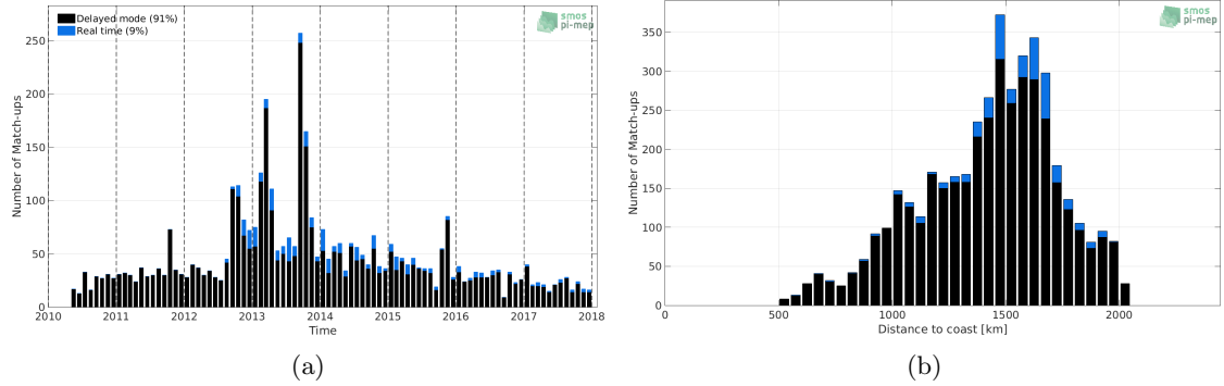
Figure 1: Number of match-ups between Argo and SMOS SSS L3 v2 - Daily - 0.5 Deg (CATDS-CECOS-IFREMER) SSS as a function of time (a) and as function of the distance to coast (b) over the SPURS 1 Pi-MEP region and for the full satellite product period.
