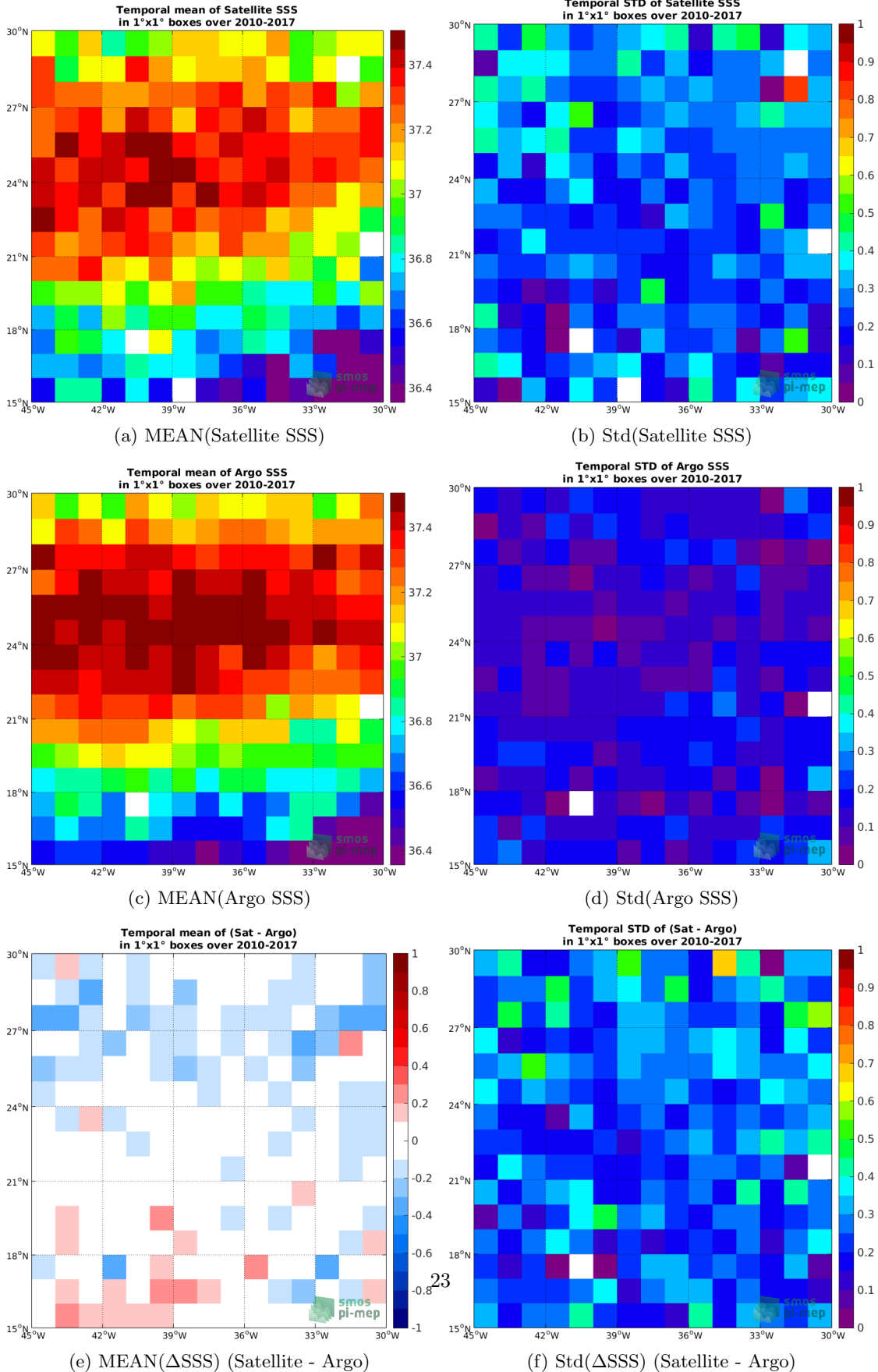
Figure 6: Temporal mean (left) and Std (right) of SSS from SMOS L3 v2 - Daily - 0.5 Deg (CATDS-CECOS-IFREMER) (top), Argo (middle), and of \Delta SSS (Satellite - Argo). Only match-up pairs are used to generate these maps.
