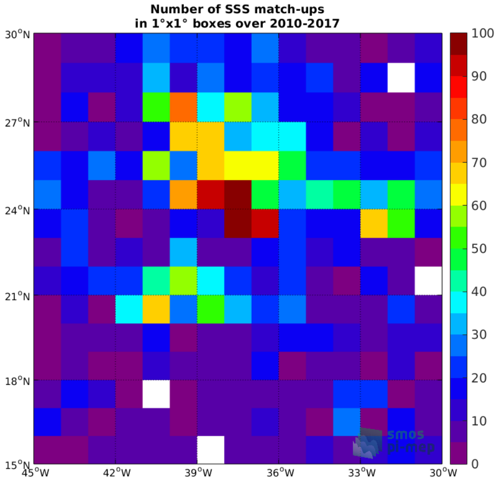
Figure 4: Number of SSS match-ups between Argo SSS and the SMOS L3 v2 - Daily - 0.5 Deg (CATDS-CECOS-IFREMER) SSS product for the SPURS 1 Pi-MEP region over 1°x1° boxes and for the full satellite product period.
