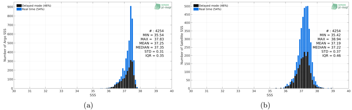
Figure 2: Histograms of SSS from Argo (a) and SMOS L3 v2 - Daily - 0.5 Deg (CATDS-CECOS-IFREMER) (b) considering all match-up pairs per bins of 0.1 over the SPURS 1 Pi-MEP region and for the full satellite product period.
