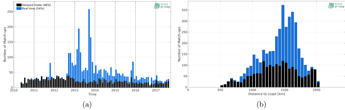
Figure 1: Number of match-ups between Argo and SMOS L3 v2 - Daily - 0.5 Deg (CATDS-CECOS-IFREMER) SSS as a function of time (a) and as function of the distance to coast (b) over the SPURS 1 Pi-MEP region and for the full satellite product period.
