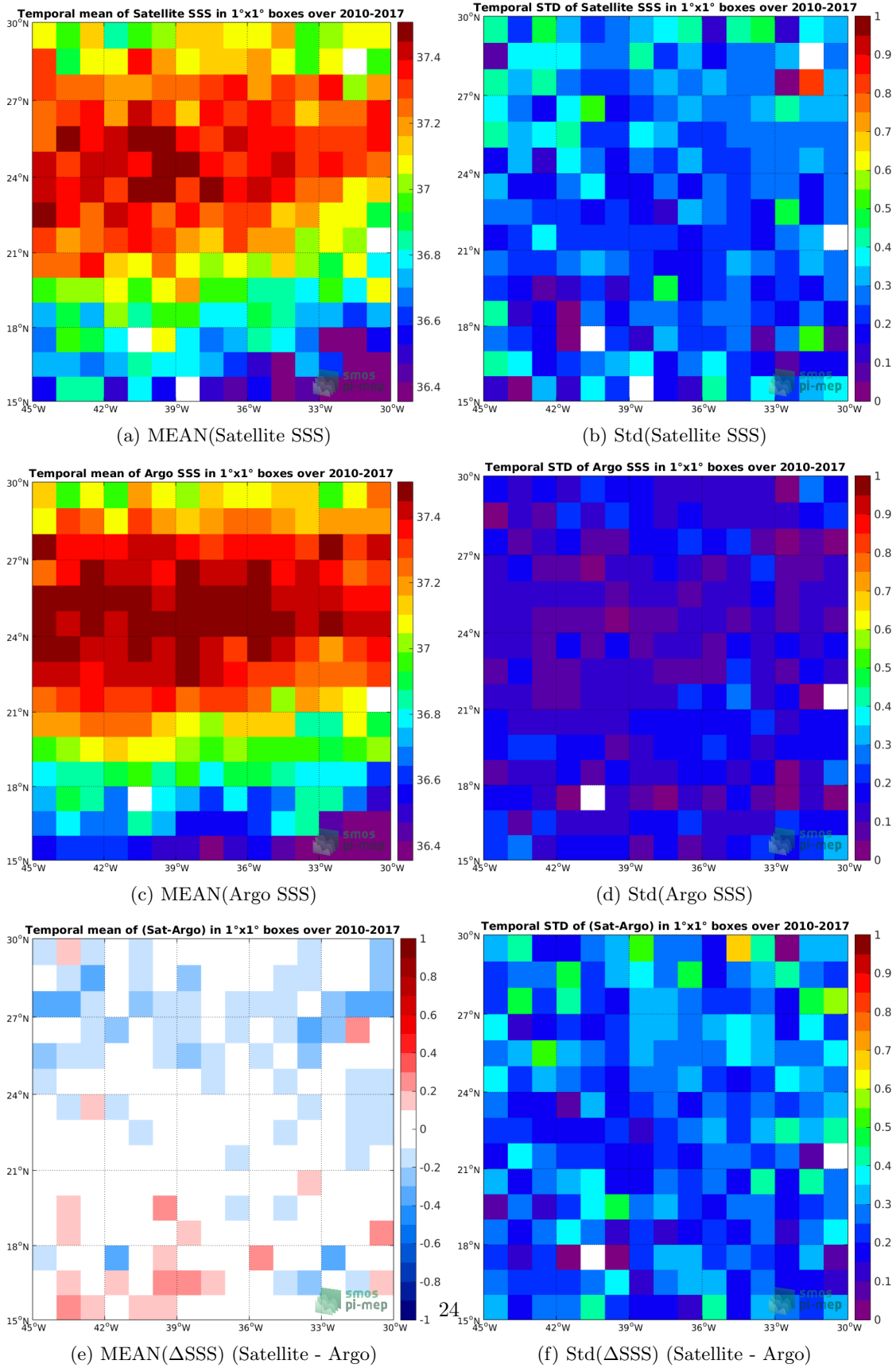
Figure 6: Temporal mean (left) and Std (right) of SSS from SMOS-L3-CATDS-CECOS-IFREMER-V2-1DAY-0.5DEG (top), Argo (middle), and of \Delta SSS (Satellite - Argo). Only match-up pairs are used to generate these maps.
