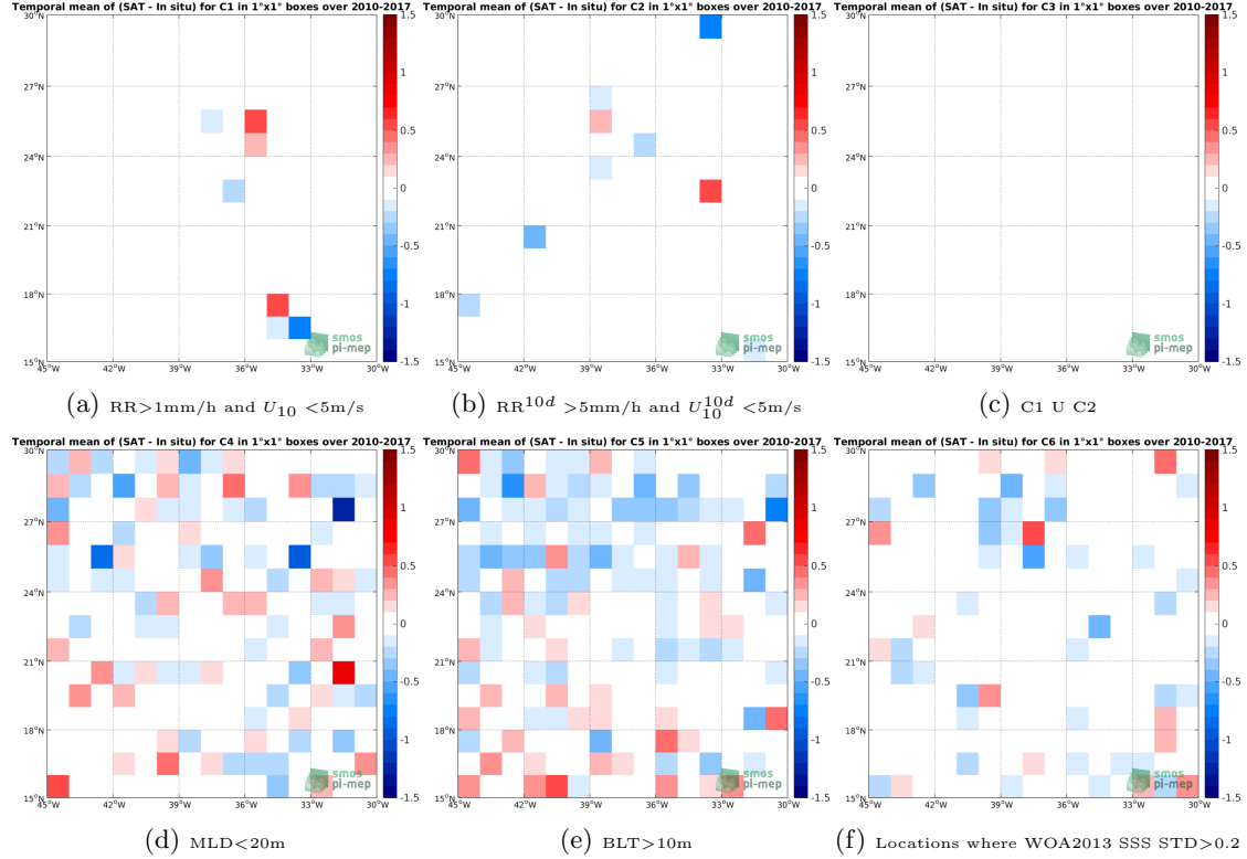
Figure 12: Temporal mean gridded over spatial boxes of size 1^\circ \times 1^\circ of \Delta\text{SSS} (SMOS-L3-CATDS-CECOS-IFREMER-V2-1DAY-0.5DEG - Argo) for 6 different subdatasets corresponding to: \text{RR} > 1\text{mm/h} and U_{10} < 5\text{m/s} (a), \text{RR}^{10d} > 5\text{mm/h} and U_{10}^{10d} < 5\text{m/s} (b), C1 U C2 (c), \text{MLD} < 20\text{m} (d), \text{BLT} > 10\text{m} (e), Locations where WOA2013 SSS STD > 0.2 (f).
