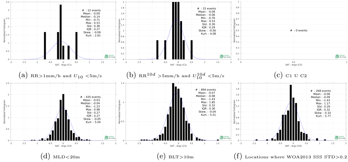
Figure 13: Normalized histogram of \Delta\text{SSS} (SMOS-L3-CATDS-CECOS-IFREMER-V2-1DAY-0.5DEG - Argo) for 6 different subdatasets corresponding to: RR>1mm/h and U_{10} < 5\text{m/s} (a), RR 10d >5mm/h and U_{10}^{10d} < 5\text{m/s} (b), C1 U C2 (c), MLD<20m (d), BLT>10m (e), Locations where WOA2013 SSS STD>0.2 (f).
