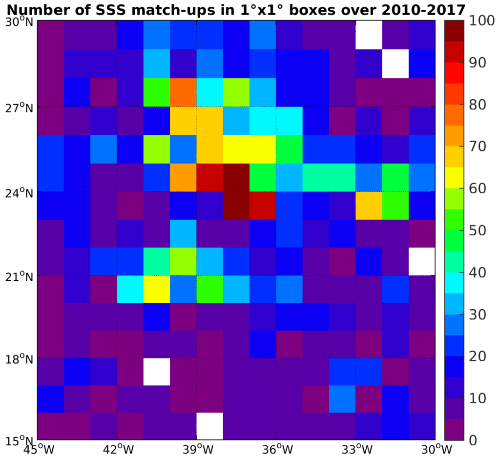
Figure 4: Number of SSS match-ups between Argo SSS and the SMOS-L3-CATDS-CECOS-IFREMER-V2-1DAY-0.5DEG SSS product for the SPURS 1 Pi-MEP region over 1°x1° boxes and for the full satellite product period.
