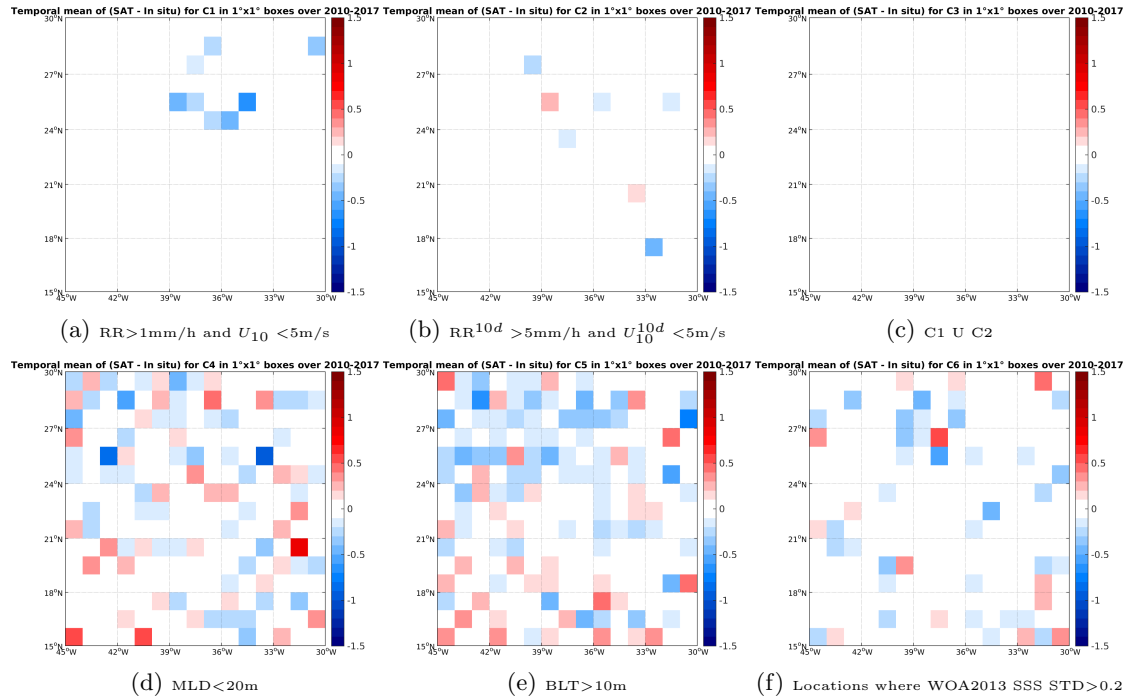
Figure 12: Temporal mean gridded over spatial boxes of size 1^\circ \times 1^\circ of \Delta SSS (SMOS-L3-CATDS-CECOS-IFREMER-V2-1DAY-0.5DEG - Argo) for 6 different subdatasets corresponding to: RR > 1\text{mm/h} and U_{10} < 5\text{m/s} (a), RR^{10d} > 5\text{mm/h} and U_{10}^{10d} < 5\text{m/s} (b), C1 U C2 (c), MLD < 20\text{m} (d), BLT > 10\text{m} (e), Locations where WOA2013 SSS STD > 0.2 (f).
