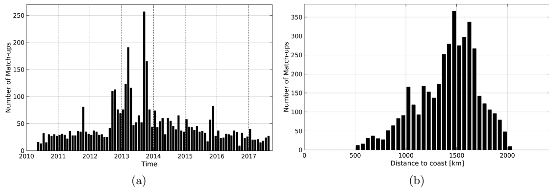
Figure 1: Number of match-ups between Argo and SMOS-L3-CATDS-CECOS-IFREMER-V2-1DAY-0.5DEG SSS as a function of time (a) and as function of the distance to coast (b) over the SPURS 1 Pi-MEP region and for the full satellite product period.
