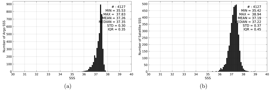
Figure 2: Histograms of SSS from Argo (a) and SMOS-L3-CATDS-CECOS-IFREMER-V2-1DAY-0.5DEG (b) considering all match-up pairs per bins of 0.1 over the SPURS 1 Pi-MEP region and for the full satellite product period.
