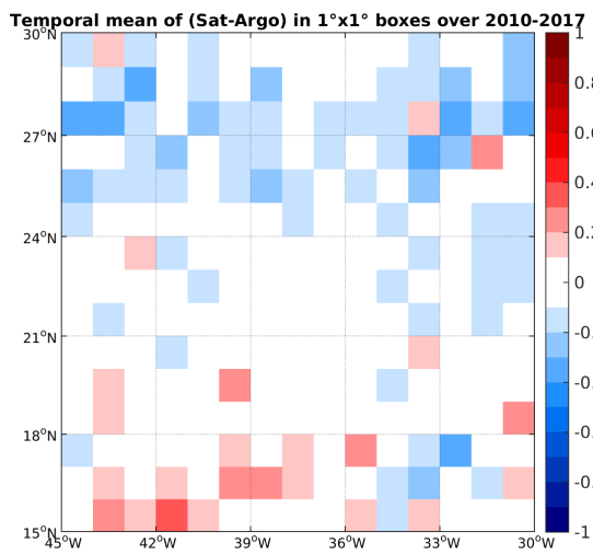
(e) MEAN( \Delta SSS) (Satellite - Argo)
