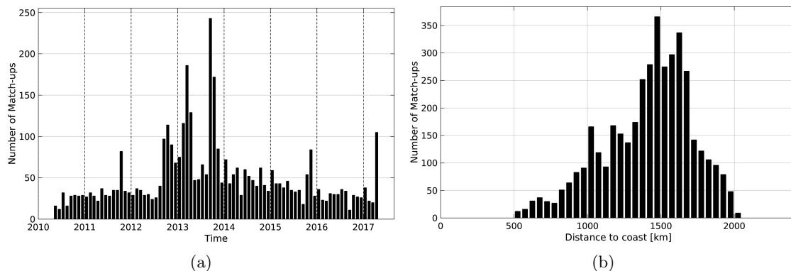
Figure 1: Number of match-ups between Argo and SMOS-L3-CATDS-CECOS-IFREMER-V2-1DAY-0.5deg SSS as a function of time (a) and as function of the distance to coast (b) over the SPURS 1 Pi-MEP region and for the full satellite product period.
