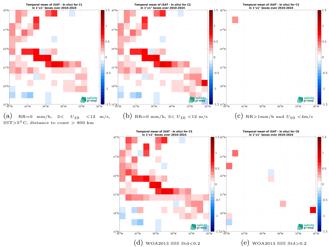
Figure 14: Temporal mean gridded over spatial boxes of size 1^\circ \times 1^\circ of \Delta\text{SSS} (SMOS SSS L3 v335 - Monthly - 25 km (CATDS-CPDC) - TSG (SAMOS)) for 5 different subdatasets corresponding to:RR=0 mm/h, 3 < U_{10} < 12 m/s, SST>5°C, distance to coast > 800 km (a), RR=0 mm/h, 3 < U_{10} < 12 m/s (b), RR>1mm/h and U_{10} < 4 m/s (c), WOA2013 SSS Std<0.2 (d), WOA2013 SSS Std>0.2 (e).
