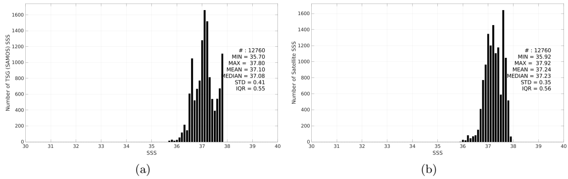
Figure 3: Histograms of SSS from TSG (SAMOS) (a) and SMOS SSS L3 v335 - Monthly - 25 km (CATDS-CPDC) (b) considering all match-up pairs per bins of 0.1 over the SPURS 1 Pi-MEP region and for the full satellite product period.
