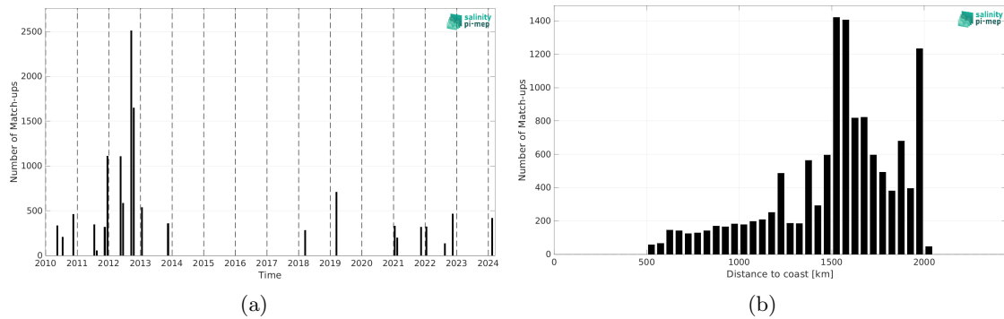
Figure 2: Number of match-ups between TSG (SAMOS) and SMOS SSS L3 v335 - Monthly - 25 km (CATDS-CPDC) SSS as a function of time (a) and as function of the distance to coast (b) over the SPURS 1 Pi-MEP region and for the full satellite product period.
