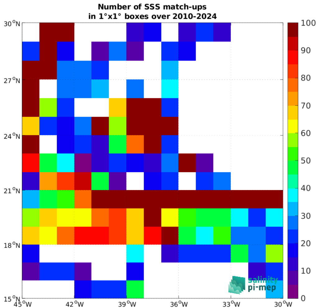
Figure 5: Number of SSS match-ups between TSG (SAMOS) SSS and the SMOS SSS L3 v335 - Monthly - 25 km (CATDS-CPDC) SSS product for the SPURS 1 Pi-MEP region over 1^\circ \times 1^\circ boxes and for the full satellite product period.
