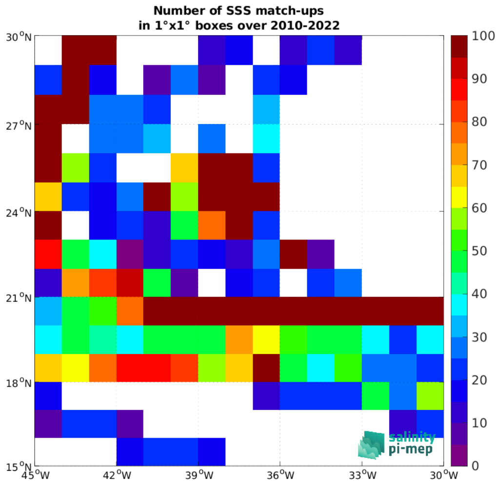
Figure 4: Number of SSS match-ups between TSG (SAMOS) SSS and the SMOS SSS L3 v335 - Monthly - 25 km (CATDS-CPDC) SSS product for the SPURS 1 Pi-MEP region over 1^\circ \times 1^\circ boxes and for the full satellite product period.
