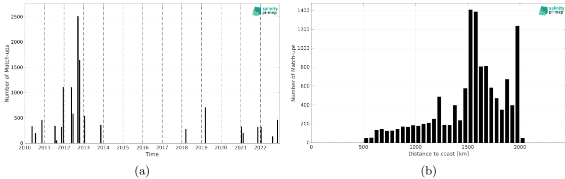
Figure 1: Number of match-ups between TSG (SAMOS) and SMOS SSS L3 v335 - Monthly - 25 km (CATDS-CPDC) SSS as a function of time (a) and as function of the distance to coast (b) over the SPURS 1 Pi-MEP region and for the full satellite product period.
