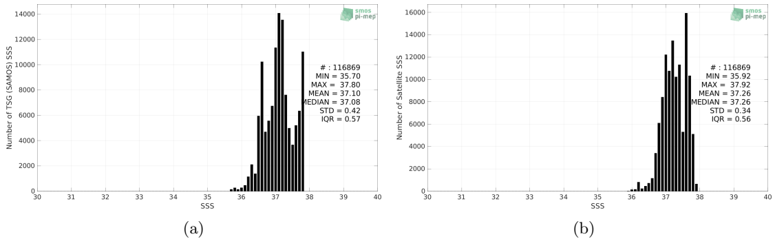
Figure 2: Histograms of SSS from TSG (SAMOS) (a) and SMOS SSS L3 v335 - Monthly - 25 km (CATDS-CPDC) (b) considering all match-up pairs per bins of 0.1 over the SPURS 1 Pi-MEP region and for the full satellite product period.
