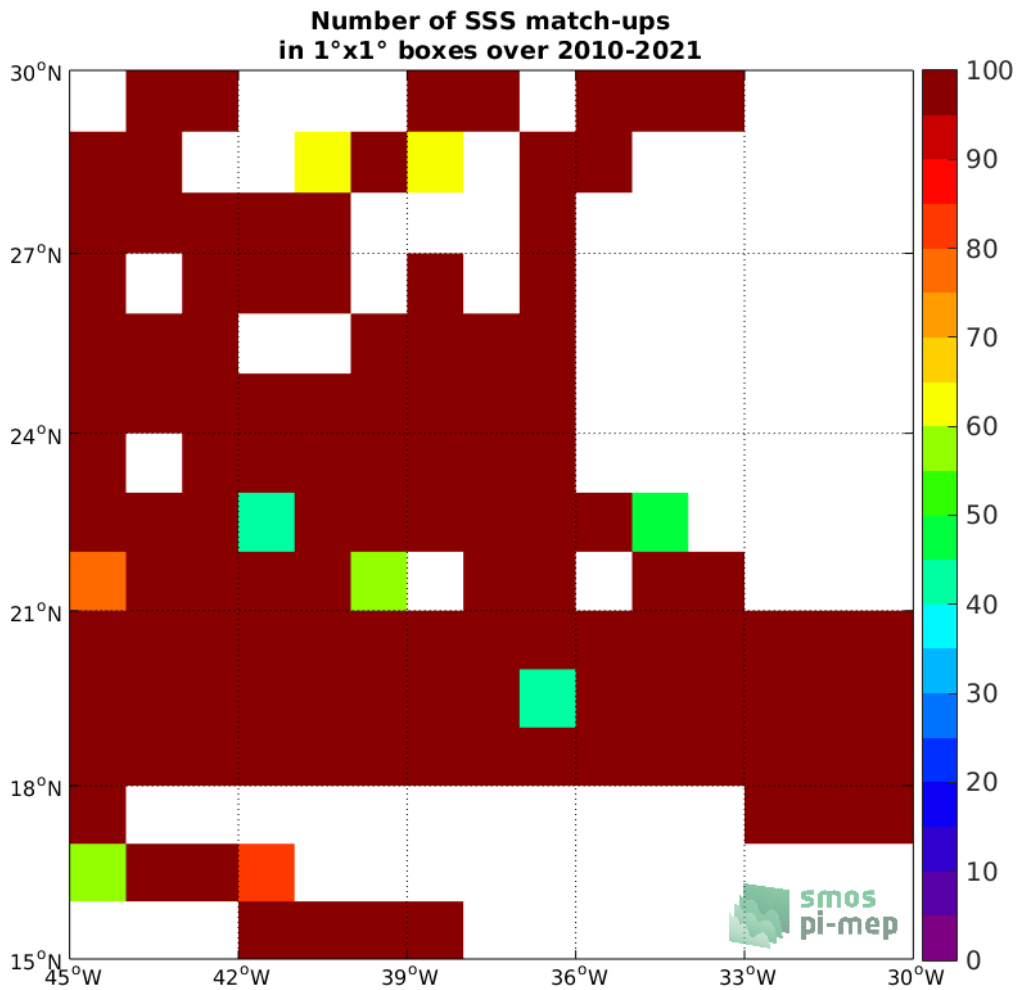
Figure 4: Number of SSS match-ups between TSG (SAMOS) SSS and the SMOS SSS L3 v335 - Monthly - 25 km (CATDS-CPDC) SSS product for the SPURS 1 Pi-MEP region over 1°×1° boxes and for the full satellite product period.
