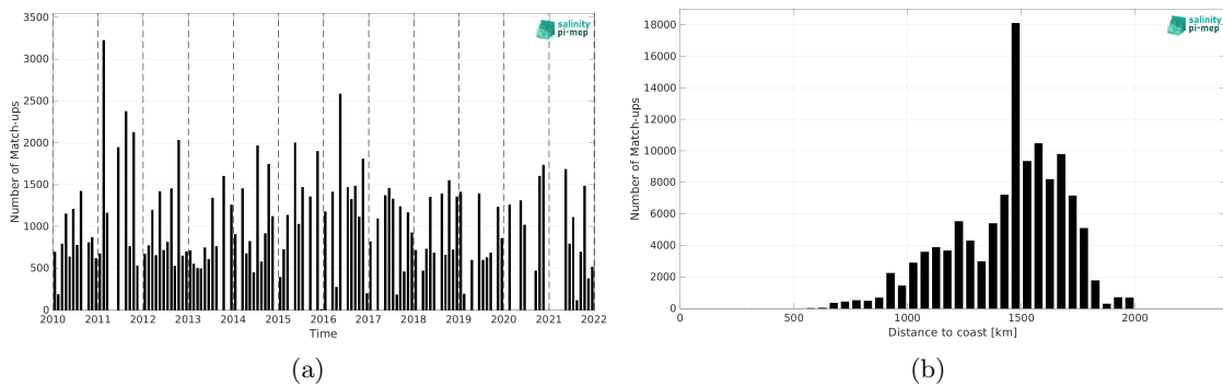
Figure 2: Number of match-ups between TSG (LEGOS-DM) and SMOS SSS L3 v335 - Monthly - 25 km (CATDS-CPDC) SSS as a function of time (a) and as function of the distance to coast (b) over the SPURS 1 Pi-MEP region and for the full satellite product period.
