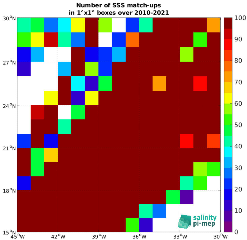
Figure 5: Number of SSS match-ups between TSG (LEGOS-DM) SSS and the SMOS SSS L3 v335 - Monthly - 25 km (CATDS-CPDC) SSS product for the SPURS 1 Pi-MEP region over 1^\circ \times 1^\circ boxes and for the full satellite product period.
