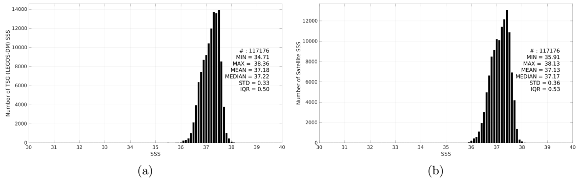
Figure 3: Histograms of SSS from TSG (LEGOS-DM) (a) and SMOS SSS L3 v335 - Monthly - 25 km (CATDS-CPDC) (b) considering all match-up pairs per bins of 0.1 over the SPURS 1 Pi-MEP region and for the full satellite product period.
