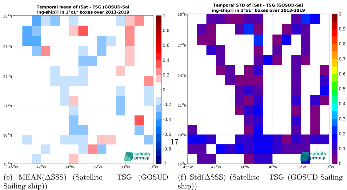
Figure 6: Temporal mean (left) and Std (right) of SSS from SMOS SSS L3 v335 - Monthly - 25 km (CATDS-CPDC) (top), TSG (GOSUD-Sailing-ship) (middle), and of \Delta SSS (Satellite - TSG (GOSUD-Sailing-ship)). Only match-up pairs are used to generate these maps.
