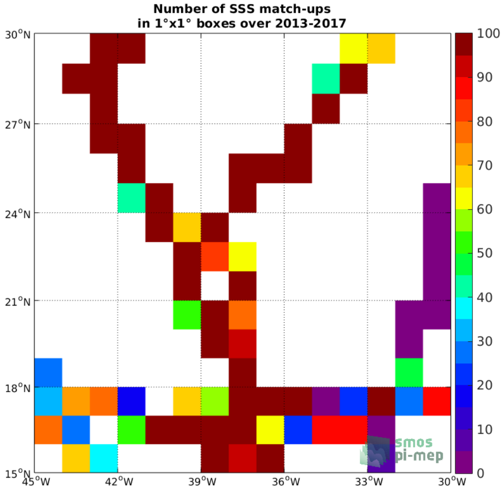
Figure 4: Number of SSS match-ups between TSG (GOSUD-Sailing-ship) SSS and the SMOS SSS L3 v335 - Monthly - 25 km (CATDS-CPDC) SSS product for the SPURS 1 Pi-MEP region over 1°x1° boxes and for the full satellite product period.
