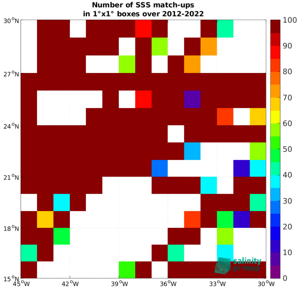
Figure 5: Number of SSS match-ups between TSG (GOSUD-Research-vessel) SSS and the SMOS SSS L3 v335 - Monthly - 25 km (CATDS-CPDC) SSS product for the SPURS 1 Pi-MEP region over 1^\circ \times 1^\circ boxes and for the full satellite product period.
