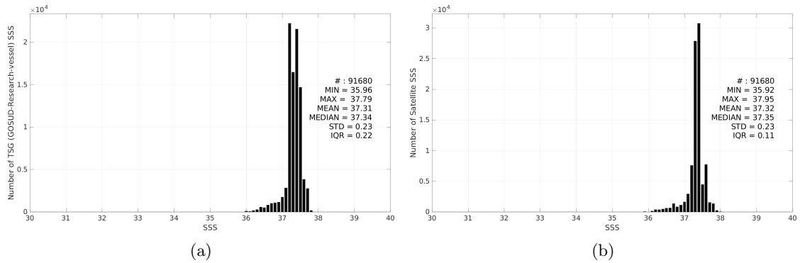
Figure 3: Histograms of SSS from TSG (GOSUD-Research-vessel) (a) and SMOS SSS L3 v335 - Monthly - 25 km (CATDS-CPDC) (b) considering all match-up pairs per bins of 0.1 over the SPURS 1 Pi-MEP region and for the full satellite product period.
