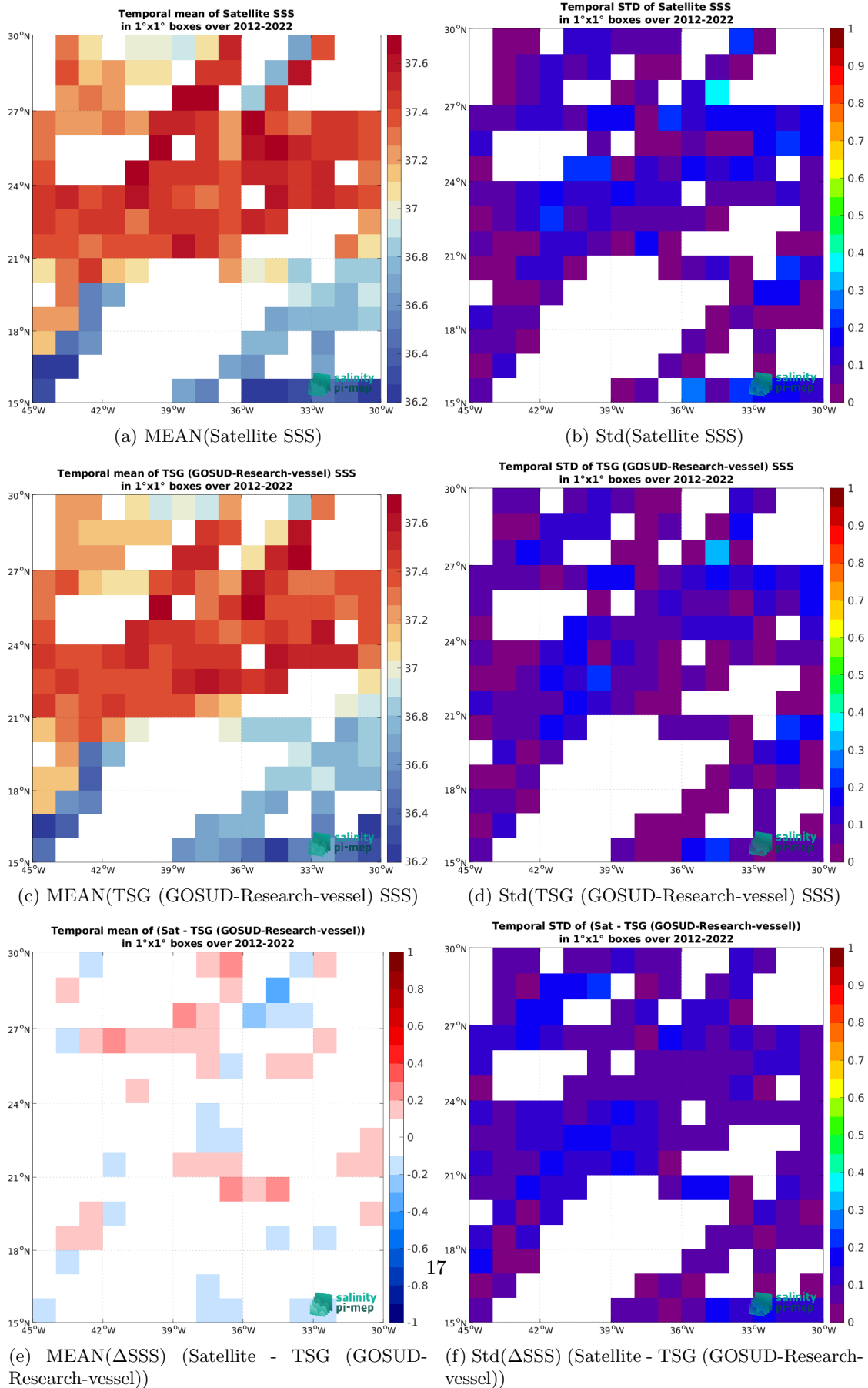
Figure 7: Temporal mean (left) and Std (right) of SSS from SMOS SSS L3 v335 - Monthly - 25 km (CATDS-CPDC) (top), TSG (GOSUD-Research-vessel) (middle), and of \Delta SSS (Satellite - TSG (GOSUD-Research-vessel)). Only match-up pairs are used to generate these maps.
