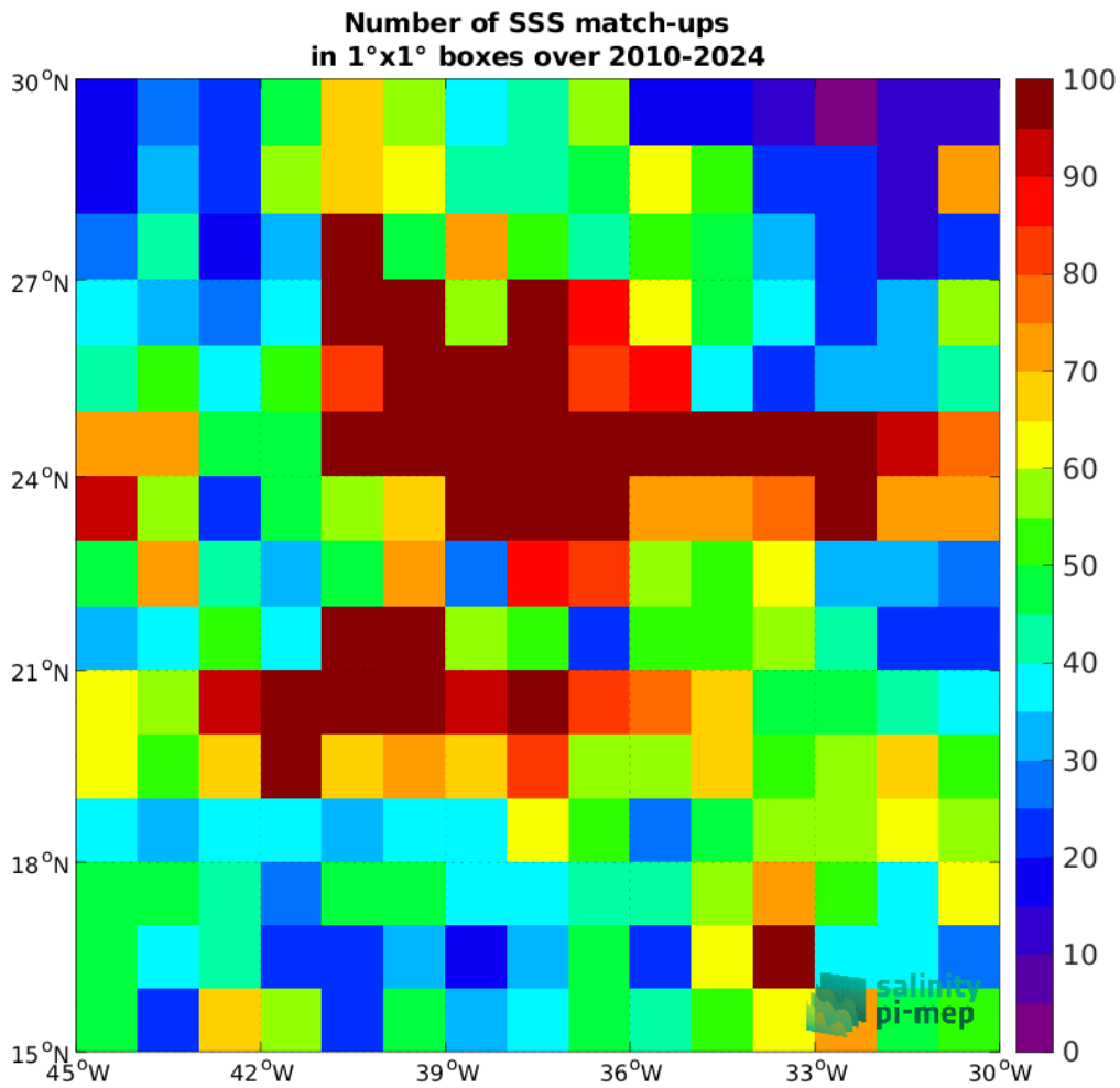
Figure 5: Number of SSS match-ups between Argo SSS and the SMOS SSS L3 v335 - Monthly - 25 km (CATDS-CPDC) SSS product for the SPURS 1 Pi-MEP region over 1^\circ \times 1^\circ boxes and for the full satellite product period.
