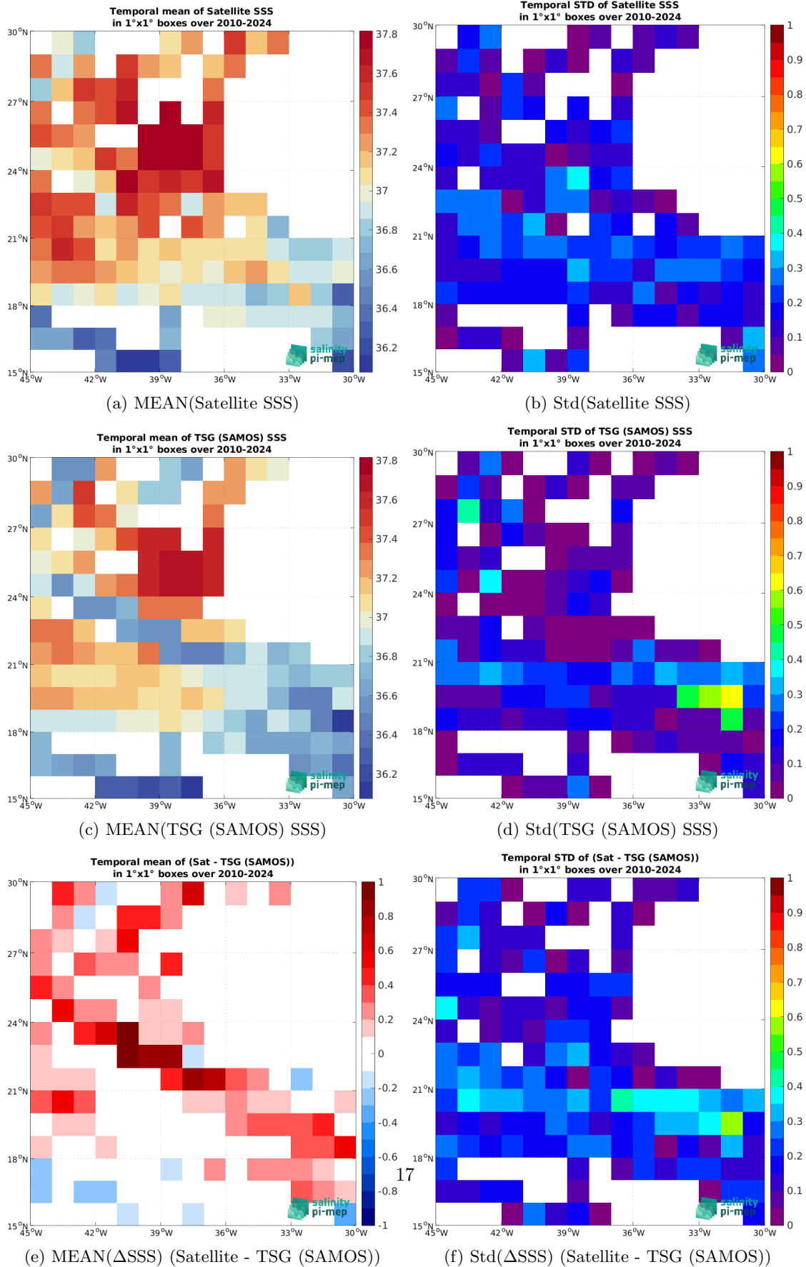
Figure 7: Temporal mean (left) and Std (right) of SSS from SMOS SSS L3 v335 - 10 Days - 25 km (CATDS-CPDC) (top), TSG (SAMOS) (middle), and of \Delta SSS (Satellite - TSG (SAMOS)). Only match-up pairs are used to generate these maps.
