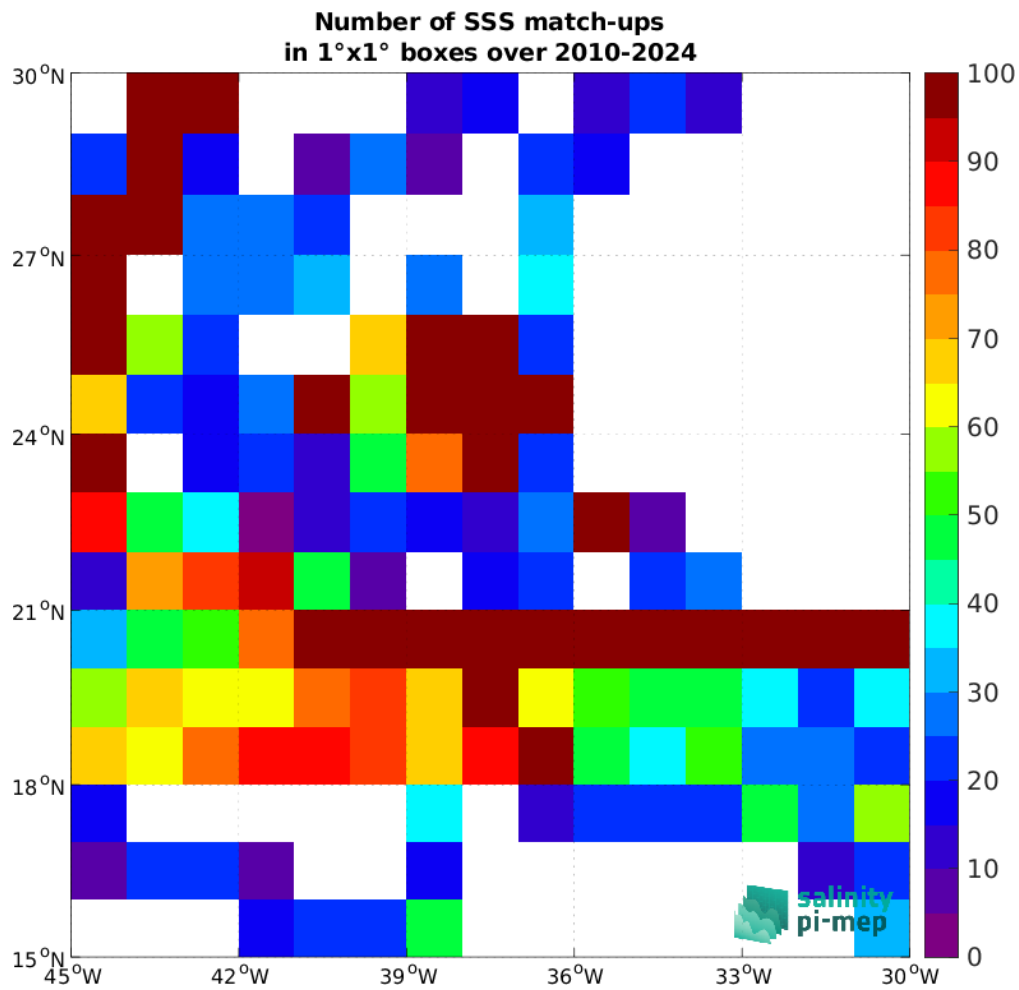
Figure 5: Number of SSS match-ups between TSG (SAMOS) SSS and the SMOS SSS L3 v335 - 10 Days - 25 km (CATDS-CPDC) SSS product for the SPURS 1 Pi-MEP region over 1^\circ \times 1^\circ boxes and for the full satellite product period.
