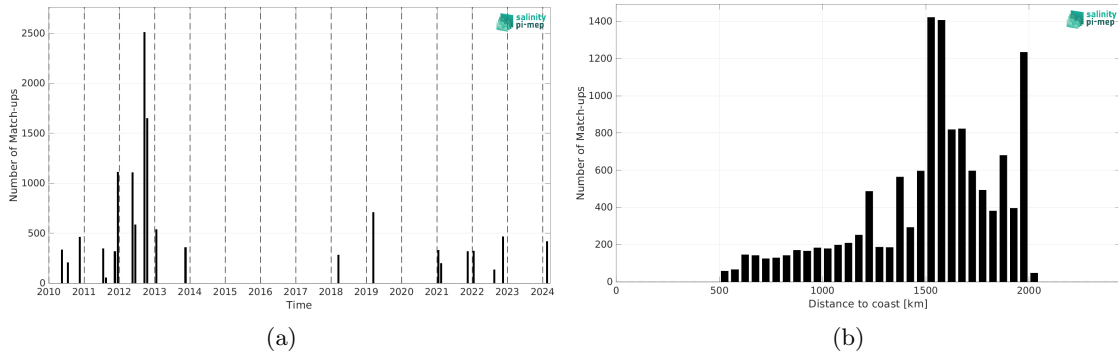
Figure 2: Number of match-ups between TSG (SAMOS) and SMOS SSS L3 v335 - 10 Days - 25 km (CATDS-CPDC) SSS as a function of time (a) and as function of the distance to coast (b) over the SPURS 1 Pi-MEP region and for the full satellite product period.
