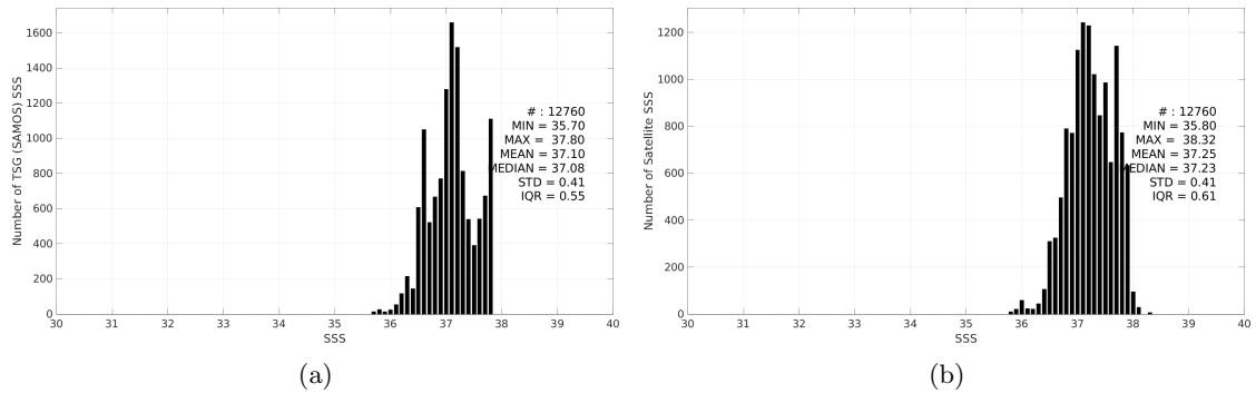
Figure 3: Histograms of SSS from TSG (SAMOS) (a) and SMOS SSS L3 v335 - 10 Days - 25 km (CATDS-CPDC) (b) considering all match-up pairs per bins of 0.1 over the SPURS 1 Pi-MEP region and for the full satellite product period.
