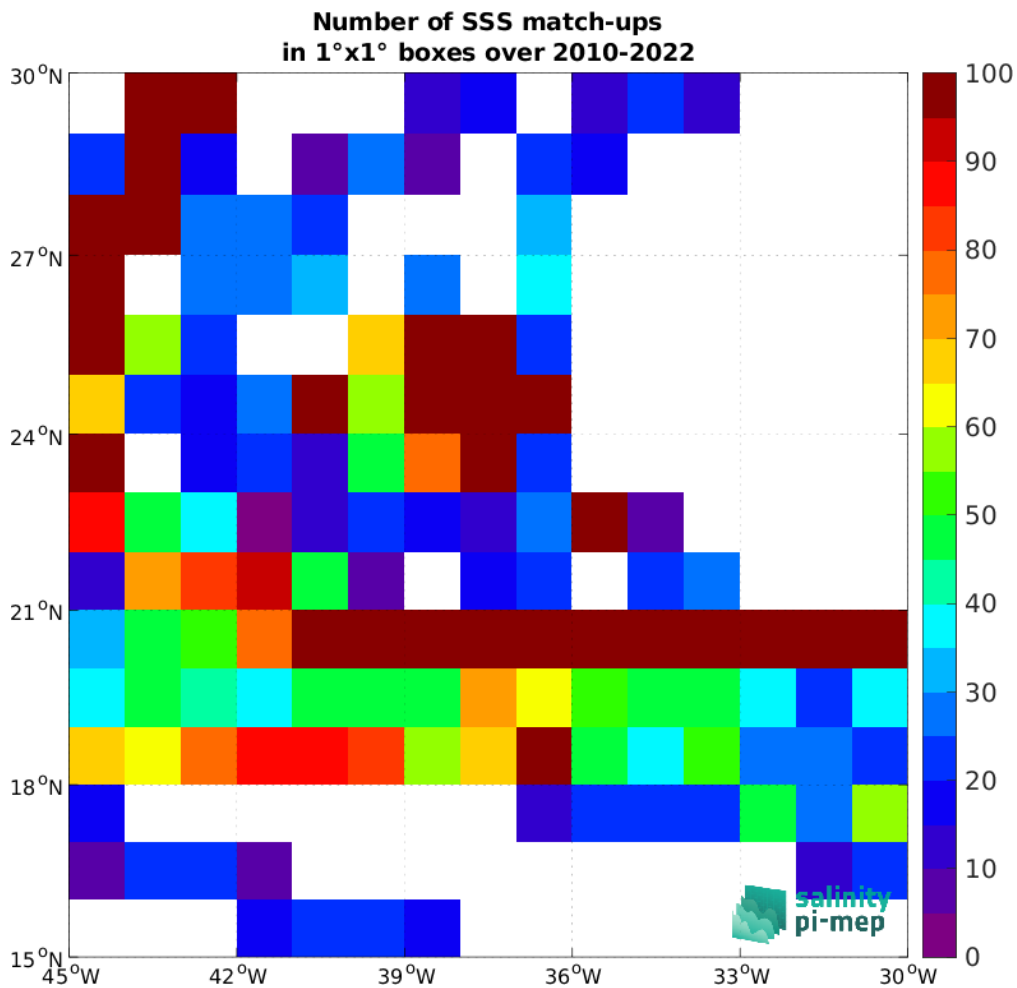
Figure 4: Number of SSS match-ups between TSG (SAMOS) SSS and the SMOS SSS L3 v335 - 10 Days - 25 km (CATDS-CPDC) SSS product for the SPURS 1 Pi-MEP region over 1^\circ \times 1^\circ boxes and for the full satellite product period.
