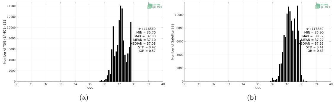
Figure 2: Histograms of SSS from TSG (SAMOS) (a) and SMOS SSS L3 v335 - 10 Days - 25 km (CATDS-CPDC) (b) considering all match-up pairs per bins of 0.1 over the SPURS 1 Pi-MEP region and for the full satellite product period.
