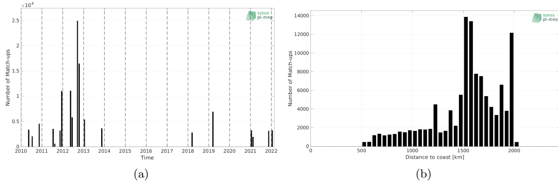
Figure 1: Number of match-ups between TSG (SAMOS) and SMOS SSS L3 v335 - 10 Days - 25 km (CATDS-CPDC) SSS as a function of time (a) and as function of the distance to coast (b) over the SPURS 1 Pi-MEP region and for the full satellite product period.
