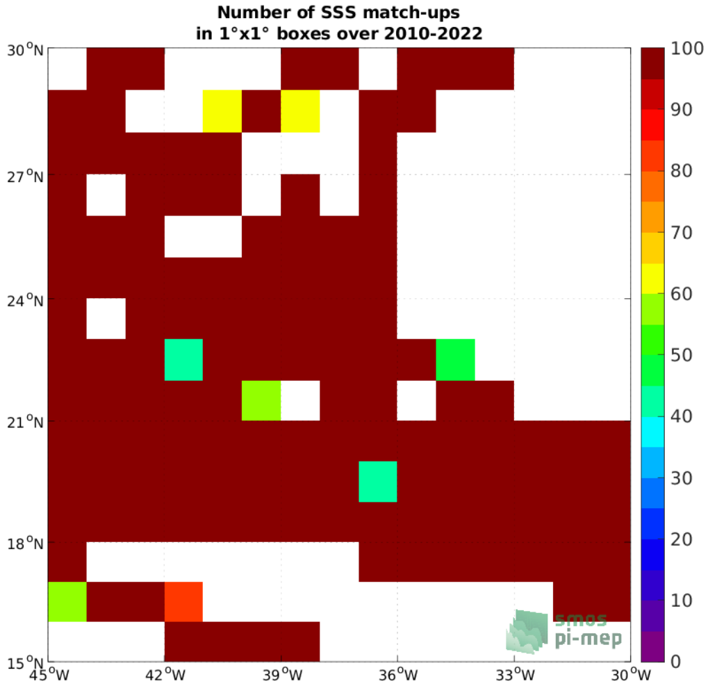
Figure 4: Number of SSS match-ups between TSG (SAMOS) SSS and the SMOS SSS L3 v335 - 10 Days - 25 km (CATDS-CPDC) SSS product for the SPURS 1 Pi-MEP region over 1°x1° boxes and for the full satellite product period.
