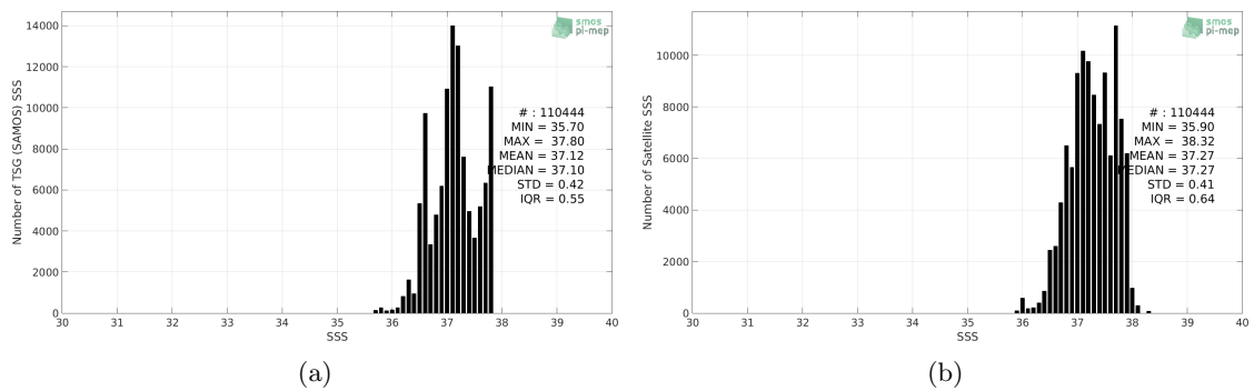
Figure 2: Histograms of SSS from TSG (SAMOS) (a) and SMOS SSS L3 v335 - 10 Days - 25 km (CATDS-CPDC) (b) considering all match-up pairs per bins of 0.1 over the SPURS 1 Pi-MEP region and for the full satellite product period.
