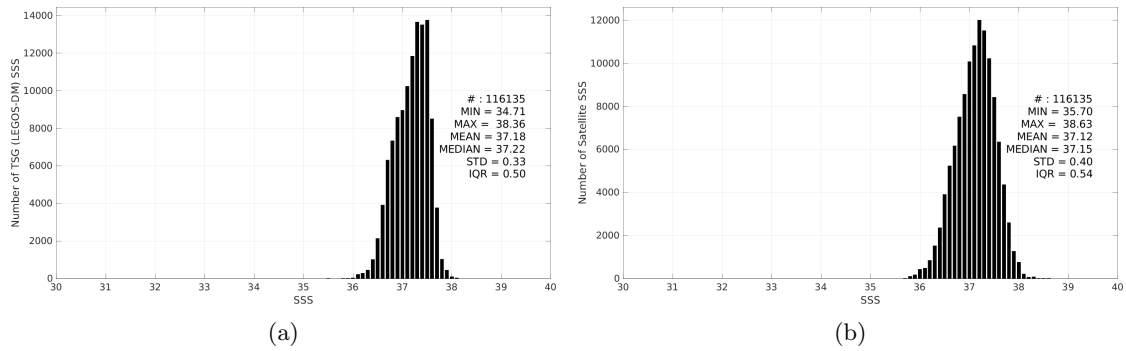
Figure 3: Histograms of SSS from TSG (LEGOS-DM) (a) and SMOS SSS L3 v335 - 10 Days - 25 km (CATDS-CPDC) (b) considering all match-up pairs per bins of 0.1 over the SPURS 1 Pi-MEP region and for the full satellite product period.
