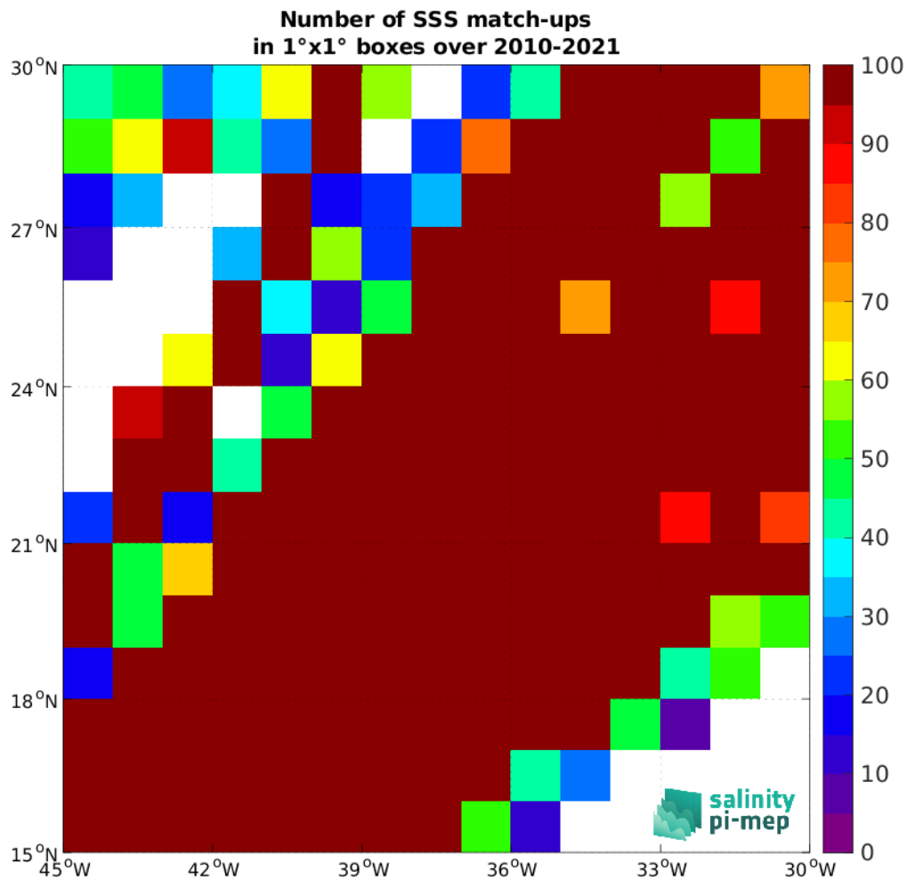
Figure 5: Number of SSS match-ups between TSG (LEGOS-DM) SSS and the SMOS SSS L3 v335 - 10 Days - 25 km (CATDS-CPDC) SSS product for the SPURS 1 Pi-MEP region over 1^\circ \times 1^\circ boxes and for the full satellite product period.
