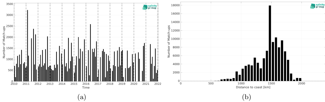
Figure 2: Number of match-ups between TSG (LEGOS-DM) and SMOS SSS L3 v335 - 10 Days - 25 km (CATDS-CPDC) SSS as a function of time (a) and as function of the distance to coast (b) over the SPURS 1 Pi-MEP region and for the full satellite product period.
