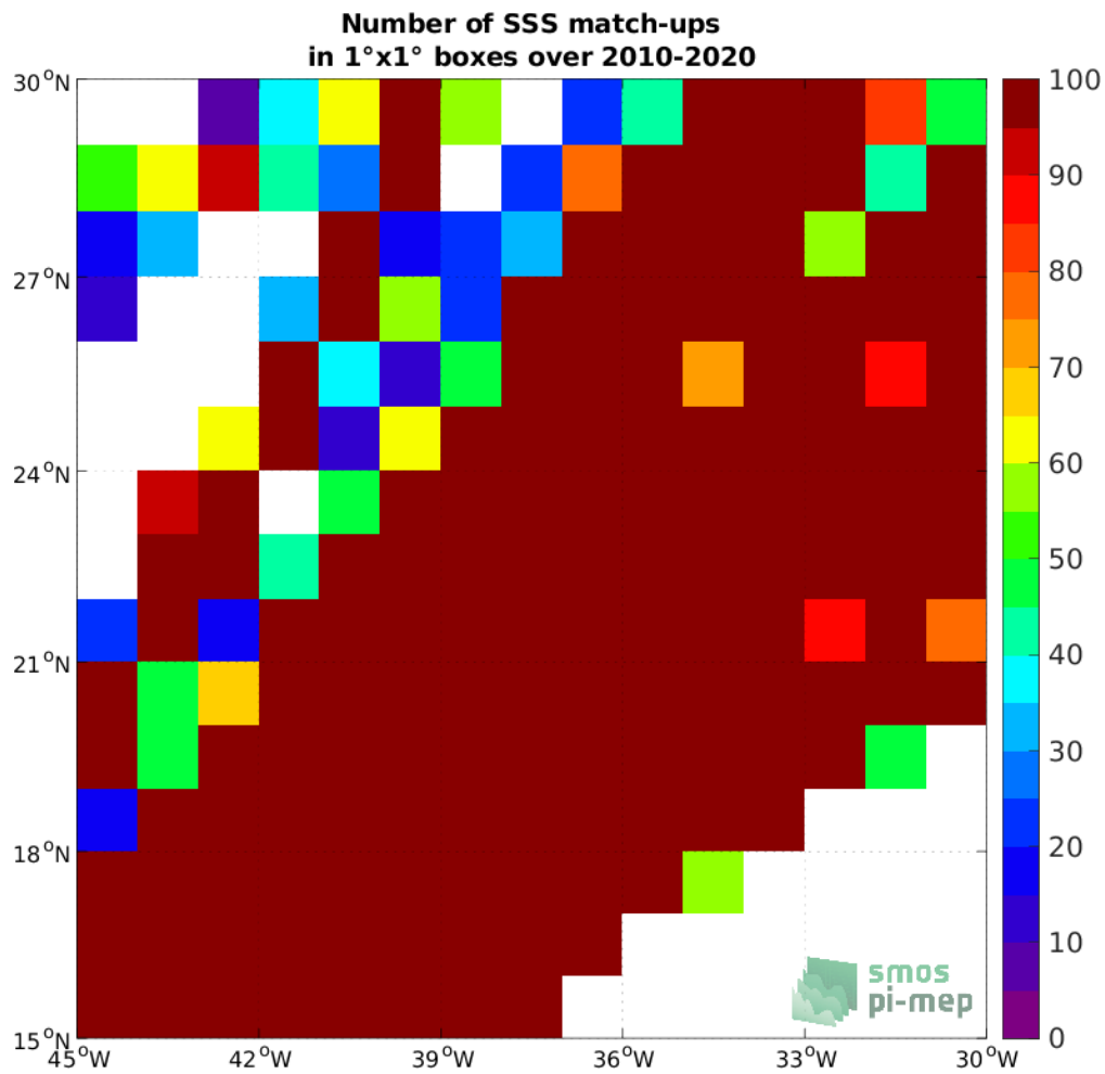
Figure 4: Number of SSS match-ups between TSG (LEGOS-DM) SSS and the SMOS SSS L3 v335 - 10 Days - 25 km (CATDS-CPDC) SSS product for the SPURS 1 Pi-MEP region over 1°x1° boxes and for the full satellite product period.
