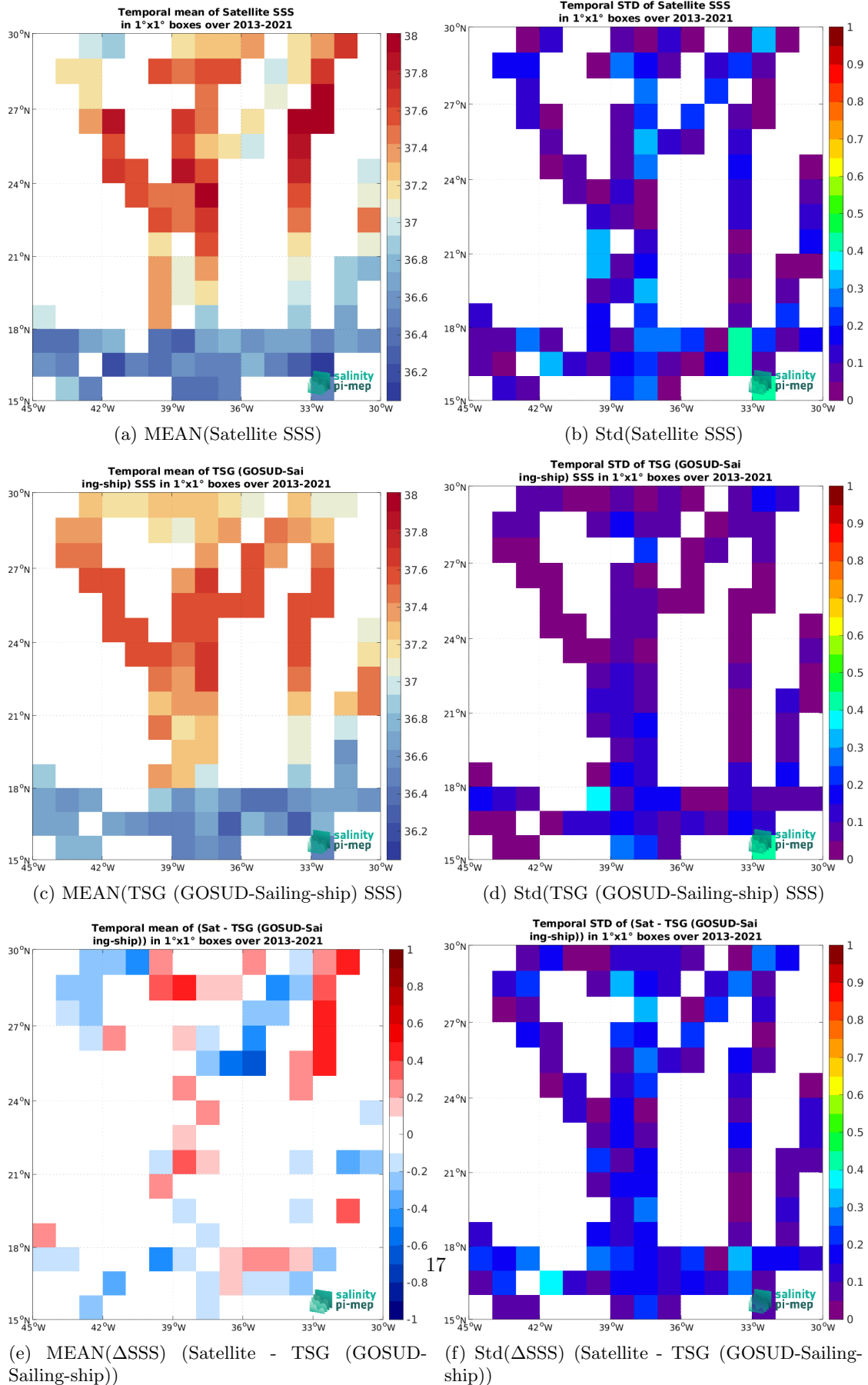
Figure 7: Temporal mean (left) and Std (right) of SSS from SMOS SSS L3 v335 - 10 Days - 25 km (CATDS-CPDC) (top), TSG (GOSUD-Sailing-ship) (middle), and of \Delta SSS (Satellite - TSG (GOSUD-Sailing-ship)). Only match-up pairs are used to generate these maps.
