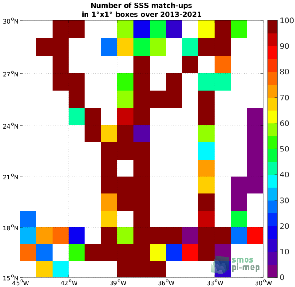
Figure 4: Number of SSS match-ups between TSG (GOSUD-Sailing-ship) SSS and the SMOS SSS L3 v335 - 10 Days - 25 km (CATDS-CPDC) SSS product for the SPURS 1 Pi-MEP region over 1^\circ \times 1^\circ boxes and for the full satellite product period.
