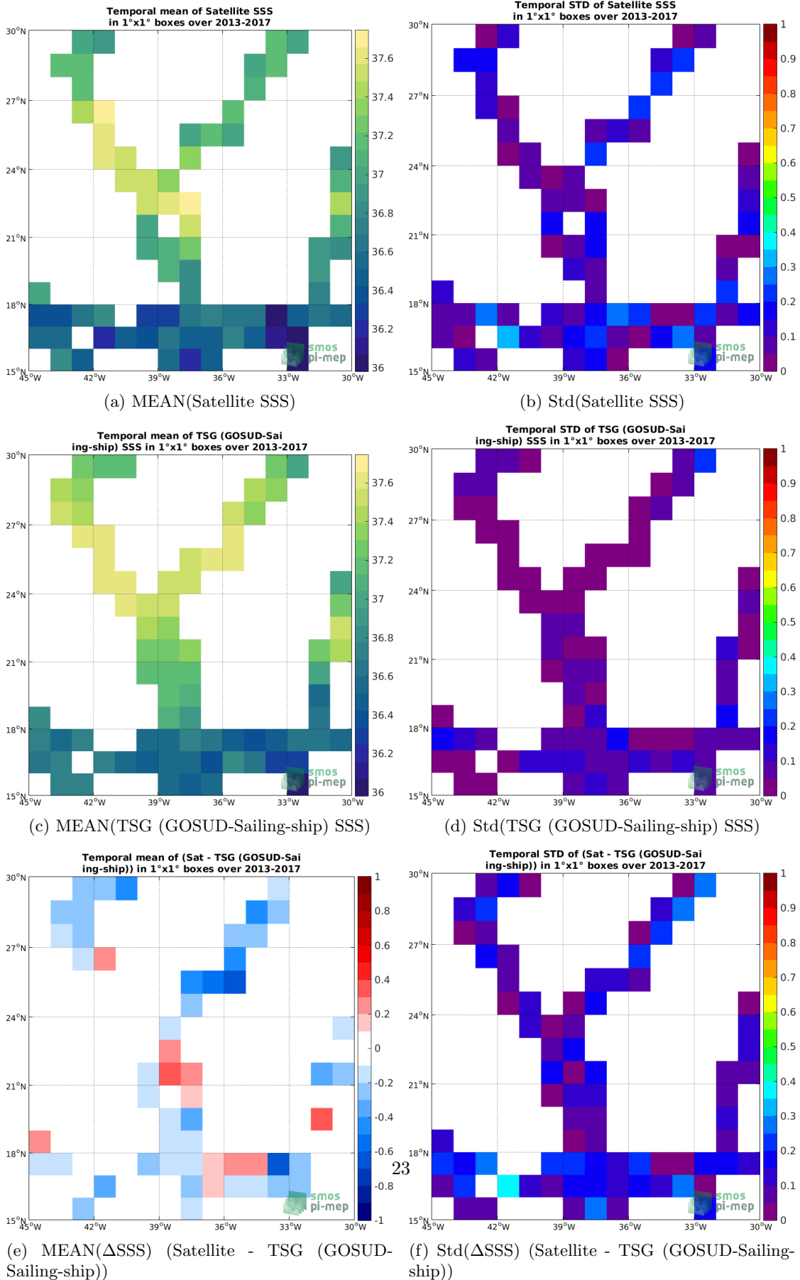
Figure 6: Temporal mean (left) and Std (right) of SSS from SMOS SSS L3 v335 - 10 Days - 25 km (CATDS-CPDC) (top), TSG (GOSUD-Sailing-ship) (middle), and of \Delta SSS (Satellite - TSG (GOSUD-Sailing-ship)). Only match-up pairs are used to generate these maps.
