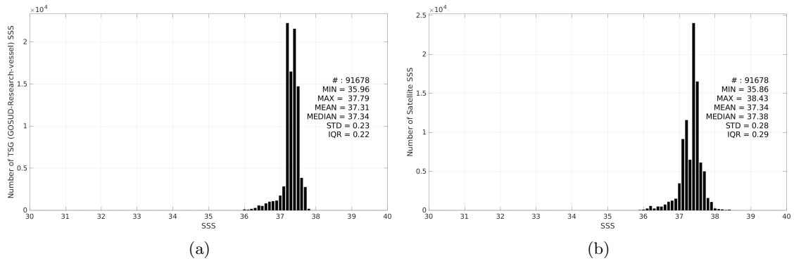
Figure 3: Histograms of SSS from TSG (GOSUD-Research-vessel) (a) and SMOS SSS L3 v335 - 10 Days - 25 km (CATDS-CPDC) (b) considering all match-up pairs per bins of 0.1 over the SPURS 1 Pi-MEP region and for the full satellite product period.
