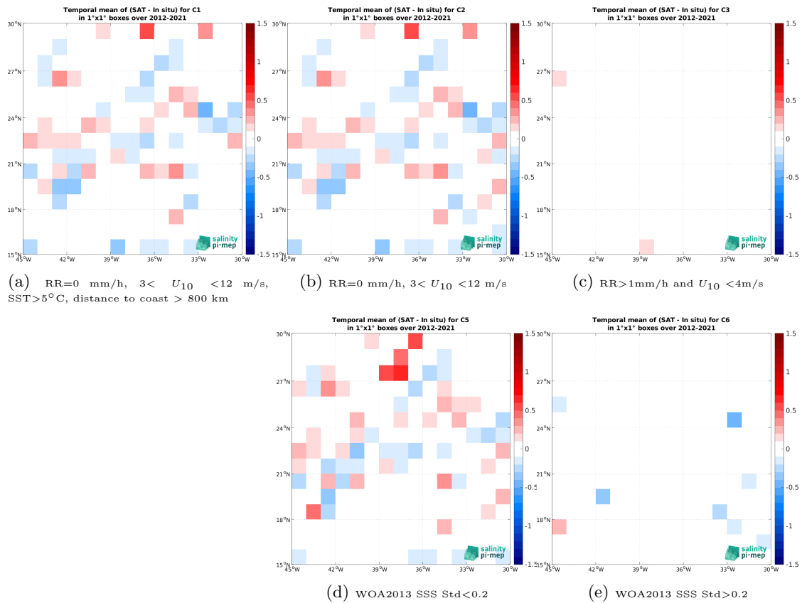
Figure 12: Temporal mean gridded over spatial boxes of size 1^{\circ} \times 1^{\circ} of \Delta\text{SSS} (SMOS SSS L3 v335 - 10 Days - 25 km (CATDS-CPDC) - TSG (GOSUD-Research-vessel)) for 5 different subdatasets corresponding to: RR=0 mm/h, 3 < U_{10} < 12 m/s, SST > 5^{\circ}\text{C} , distance to coast > 800 km (a), RR=0 mm/h, 3 < U_{10} < 12 m/s (b), RR > 1\text{mm/h} and U_{10} < 4\text{m/s} (c), WOA2013 SSS Std < 0.2 (d), WOA2013 SSS Std > 0.2 (e).
