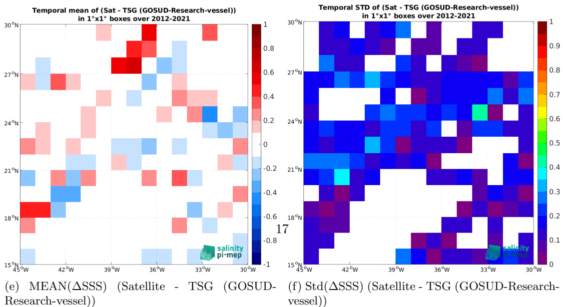
Figure 6: Temporal mean (left) and Std (right) of SSS from SMOS SSS L3 v335 - 10 Days - 25 km (CATDS-CPDC) (top), TSG (GOSUD-Research-vessel) (middle), and of \Delta SSS (Satellite - TSG (GOSUD-Research-vessel)). Only match-up pairs are used to generate these maps.
