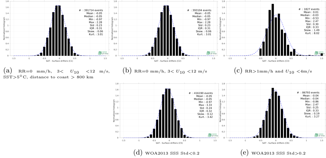
Figure 12: Normalized histogram of \Delta\text{SSS} (SMOS SSS L3 v335 - 10 Days - 25 km (CATDS-CPDC) - Surface drifters) for 5 different subdatasets corresponding to: RR=0 mm/h, 3 < U_{10} < 12 m/s, SST>5°C, distance to coast > 800 km (a), RR=0 mm/h, 3 < U_{10} < 12 m/s (b), RR>1mm/h and U_{10} < 4 m/s (c), WOA2013 SSS Std<0.2 (d), WOA2013 SSS Std>0.2 (e).
