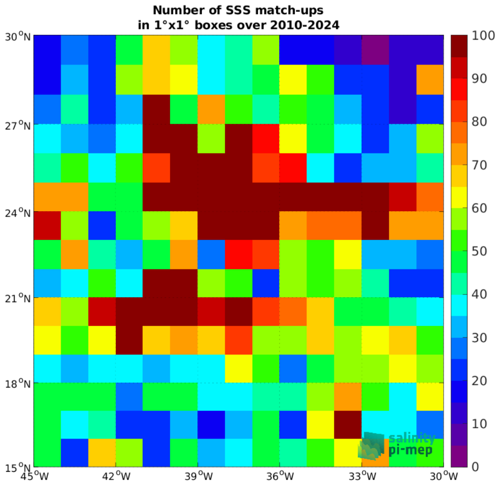
Figure 5: Number of SSS match-ups between Argo SSS and the SMOS SSS L3 v335 - 10 Days - 25 km (CATDS-CPDC) SSS product for the SPURS 1 Pi-MEP region over 1^\circ \times 1^\circ boxes and for the full satellite product period.
