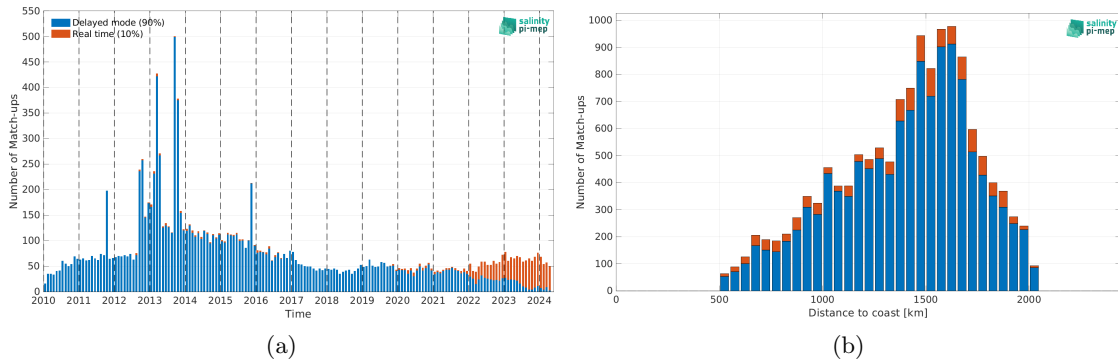
Figure 2: Number of match-ups between Argo and SMOS SSS L3 v335 - 10 Days - 25 km (CATDS-CPDC) SSS as a function of time (a) and as function of the distance to coast (b) over the SPURS 1 Pi-MEP region and for the full satellite product period.
