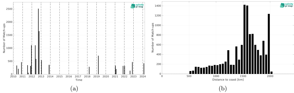
Figure 2: Number of match-ups between TSG (SAMOS) and SMOS SSS L3 v332 - 9 Days (CATDS-CPDC) SSS as a function of time (a) and as function of the distance to coast (b) over the SPURS 1 Pi-MEP region and for the full satellite product period.
