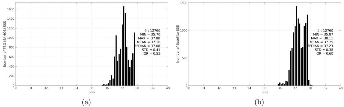
Figure 3: Histograms of SSS from TSG (SAMOS) (a) and SMOS SSS L3 v332 - 9 Days (CATDS-CPDC) (b) considering all match-up pairs per bins of 0.1 over the SPURS 1 Pi-MEP region and for the full satellite product period.
