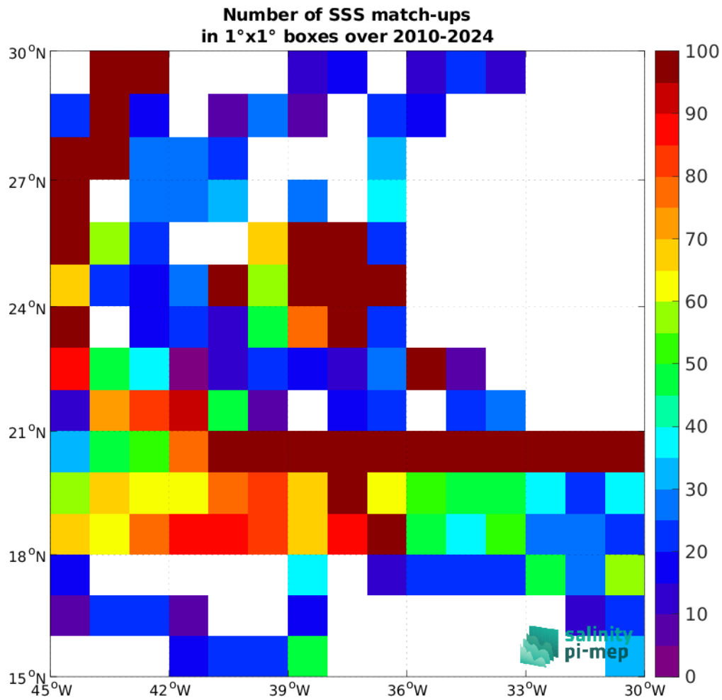
Figure 5: Number of SSS match-ups between TSG (SAMOS) SSS and the SMOS SSS L3 v332 - 9 Days (CATDS-CPDC) SSS product for the SPURS 1 Pi-MEP region over 1^\circ \times 1^\circ boxes and for the full satellite product period.
