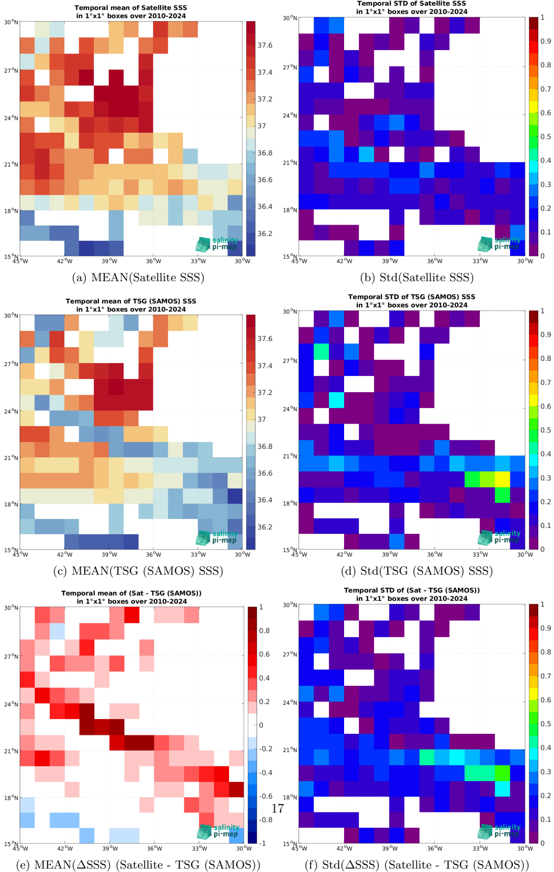
Figure 7: Temporal mean (left) and Std (right) of SSS from SMOS SSS L3 v332 - 9 Days (CATDS-CPDC) (top), TSG (SAMOS) (middle), and of \Delta SSS (Satellite - TSG (SAMOS)). Only match-up pairs are used to generate these maps.
