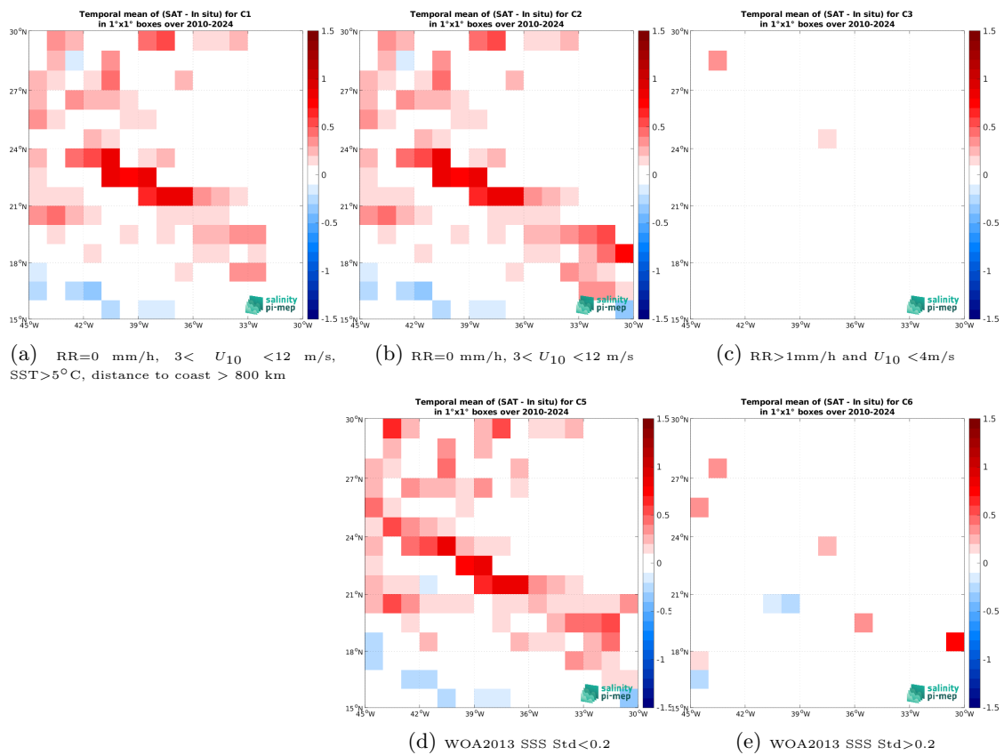
Figure 14: Temporal mean gridded over spatial boxes of size 1^\circ \times 1^\circ of \Delta SSS (SMOS SSS L3 v332 - 9 Days (CATDS-CPDC) - TSG (SAMOS)) for 5 different subdatasets corresponding to: RR=0 mm/h, 3 < U_{10} < 12 m/s, SST > 5^\circ C , distance to coast > 800 km (a), RR=0 mm/h, 3 < U_{10} < 12 m/s (b), RR > 1 mm/h and U_{10} < 4 m/s (c), WOA2013 SSS Std < 0.2 (d), WOA2013 SSS Std > 0.2 (e).
