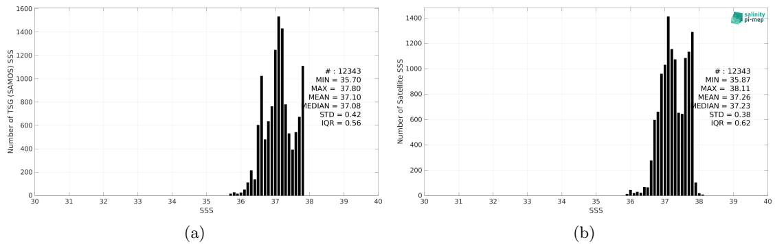
Figure 2: Histograms of SSS from TSG (SAMOS) (a) and SMOS SSS L3 v332 - 9 Days (CATDS-CPDC) (b) considering all match-up pairs per bins of 0.1 over the SPURS 1 Pi-MEP region and for the full satellite product period.
