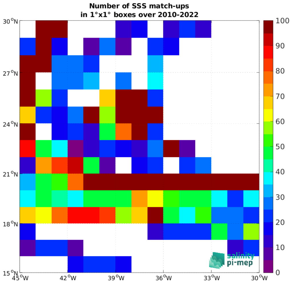
Figure 4: Number of SSS match-ups between TSG (SAMOS) SSS and the SMOS SSS L3 v332 - 9 Days (CATDS-CPDC) SSS product for the SPURS 1 Pi-MEP region over 1°x1° boxes and for the full satellite product period.
