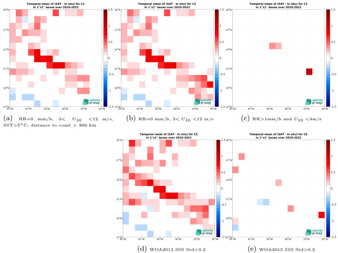
Figure 12: Temporal mean gridded over spatial boxes of size 1^\circ \times 1^\circ of \Delta SSS (SMOS SSS L3 v332 - 9 Days (CATDS-CPDC) - TSG (SAMOS)) for 5 different subdatasets corresponding to: RR=0 mm/h, 3 < U_{10} < 12 m/s, SST > 5^\circ\text{C} , distance to coast > 800 km (a), RR=0 mm/h, 3 < U_{10} < 12 m/s (b), RR > 1 mm/h and U_{10} < 4 m/s (c), WOA2013 SSS Std < 0.2 (d), WOA2013 SSS Std > 0.2 (e).
