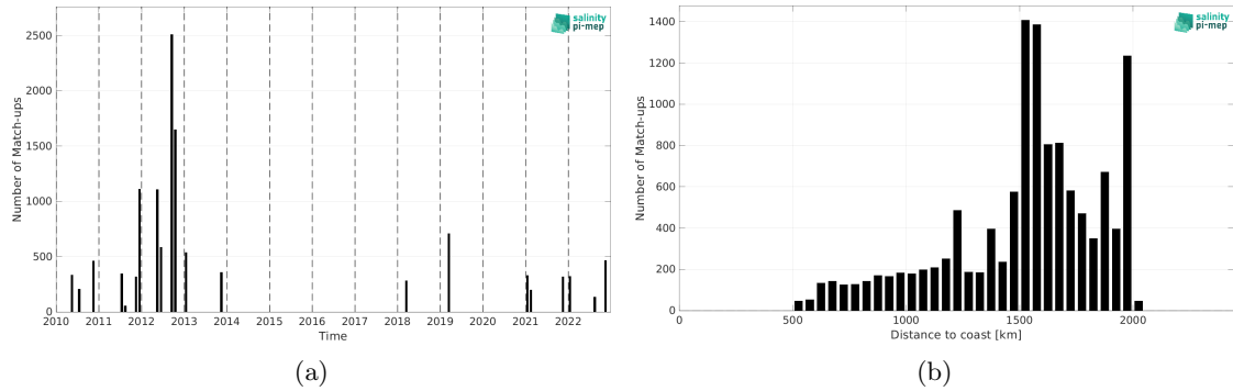
Figure 1: Number of match-ups between TSG (SAMOS) and SMOS SSS L3 v332 - 9 Days (CATDS-CPDC) SSS as a function of time (a) and as function of the distance to coast (b) over the SPURS 1 Pi-MEP region and for the full satellite product period.
