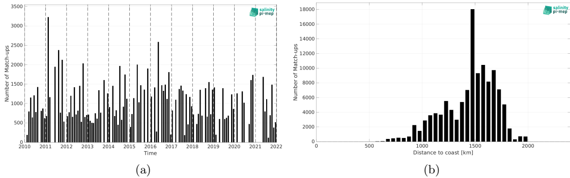
Figure 2: Number of match-ups between TSG (LEGOS-DM) and SMOS SSS L3 v332 - 9 Days (CATDS-CPDC) SSS as a function of time (a) and as function of the distance to coast (b) over the SPURS 1 Pi-MEP region and for the full satellite product period.
