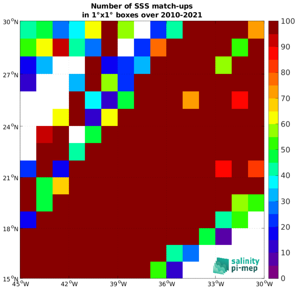
Figure 5: Number of SSS match-ups between TSG (LEGOS-DM) SSS and the SMOS SSS L3 v332 - 9 Days (CATDS-CPDC) SSS product for the SPURS 1 Pi-MEP region over 1°x1° boxes and for the full satellite product period.
