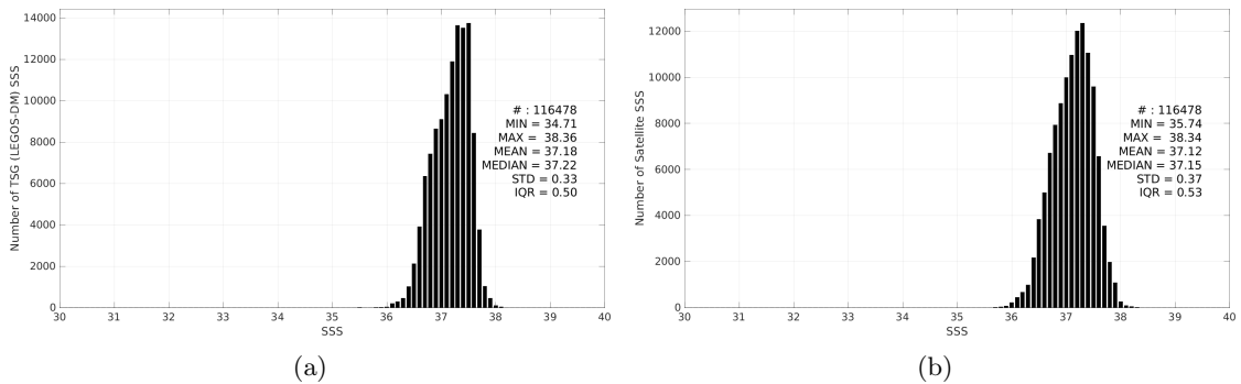
Figure 3: Histograms of SSS from TSG (LEGOS-DM) (a) and SMOS SSS L3 v332 - 9 Days (CATDS-CPDC) (b) considering all match-up pairs per bins of 0.1 over the SPURS 1 Pi-MEP region and for the full satellite product period.
