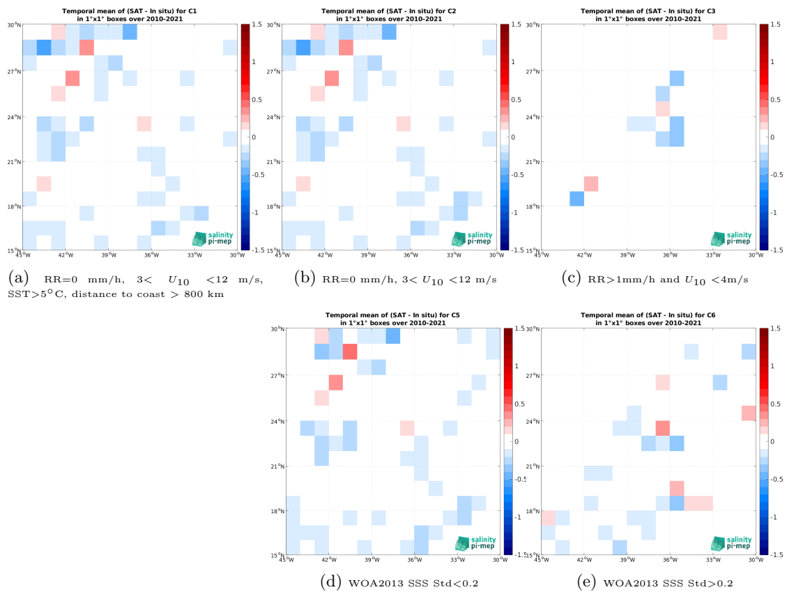
Figure 14: Temporal mean gridded over spatial boxes of size 1^\circ \times 1^\circ of \Delta SSS (SMOS SSS L3 v332 - 9 Days (CATDS-CPDC) - TSG (LEGOS-DM)) for 5 different subdatasets corresponding to: RR=0 mm/h, 3 < U_{10} < 12 m/s, SST > 5^\circ C , distance to coast > 800 km (a), RR=0 mm/h, 3 < U_{10} < 12 m/s (b), RR > 1 mm/h and U_{10} < 4 m/s (c), WOA2013 SSS Std < 0.2 (d), WOA2013 SSS Std > 0.2 (e).
