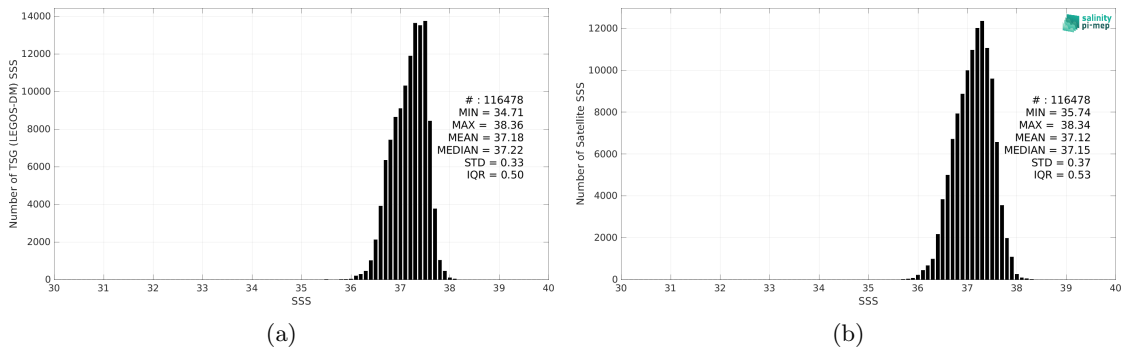
Figure 2: Histograms of SSS from TSG (LEGOS-DM) (a) and SMOS SSS L3 v332 - 9 Days (CATDS-CPDC) (b) considering all match-up pairs per bins of 0.1 over the SPURS 1 Pi-MEP region and for the full satellite product period.
