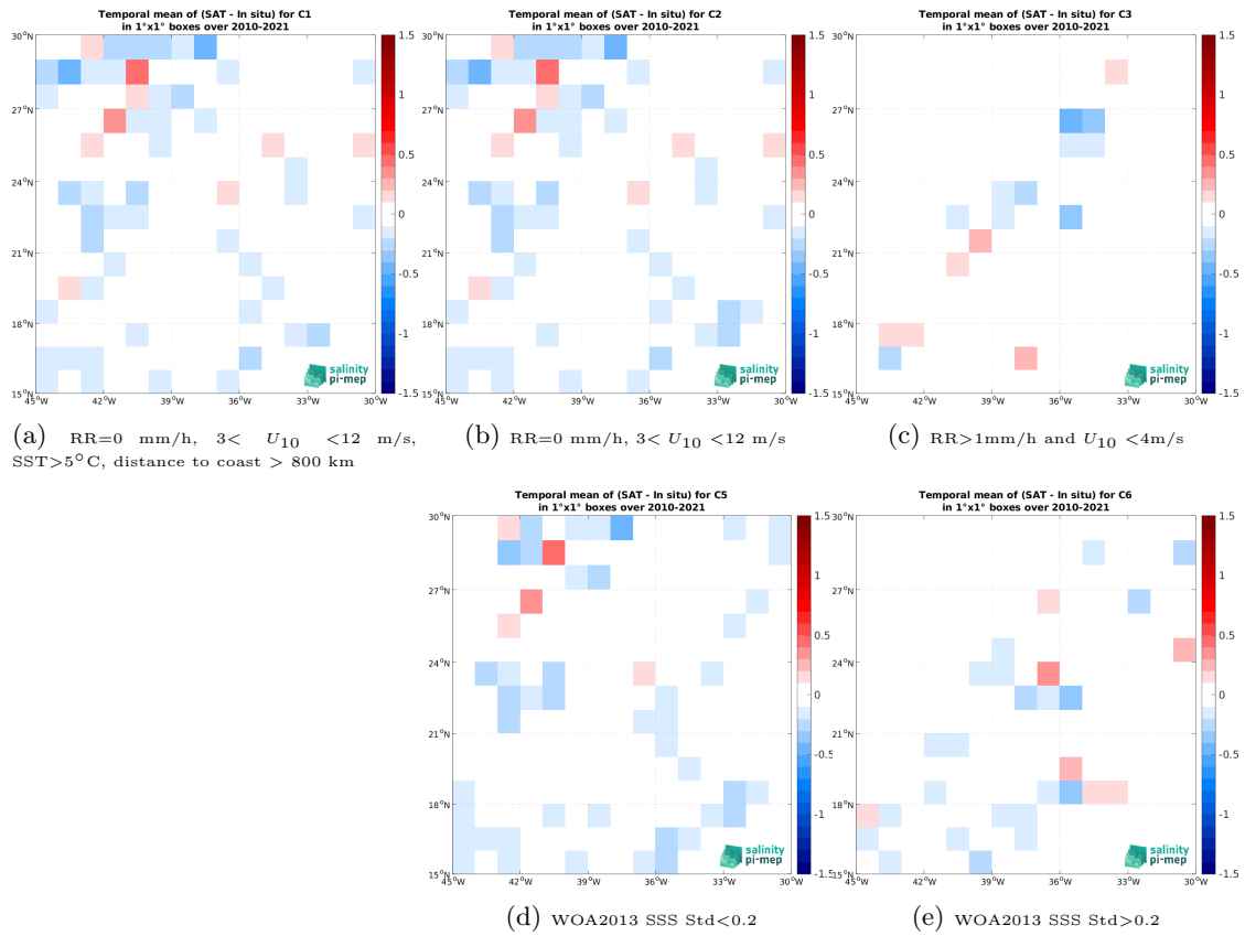
Figure 12: Temporal mean gridded over spatial boxes of size 1^\circ \times 1^\circ of \Delta SSS (SMOS SSS L3 v332 - 9 Days (CATDS-CPDC) - TSG (LEGOS-DM)) for 5 different subdatasets corresponding to: RR=0 mm/h, 3 < U_{10} < 12 m/s, SST > 5^\circ C , distance to coast > 800 km (a), RR=0 mm/h, 3 < U_{10} < 12 m/s (b), RR > 1 mm/h and U_{10} < 4 m/s (c), WOA2013 SSS Std < 0.2 (d), WOA2013 SSS Std > 0.2 (e).
