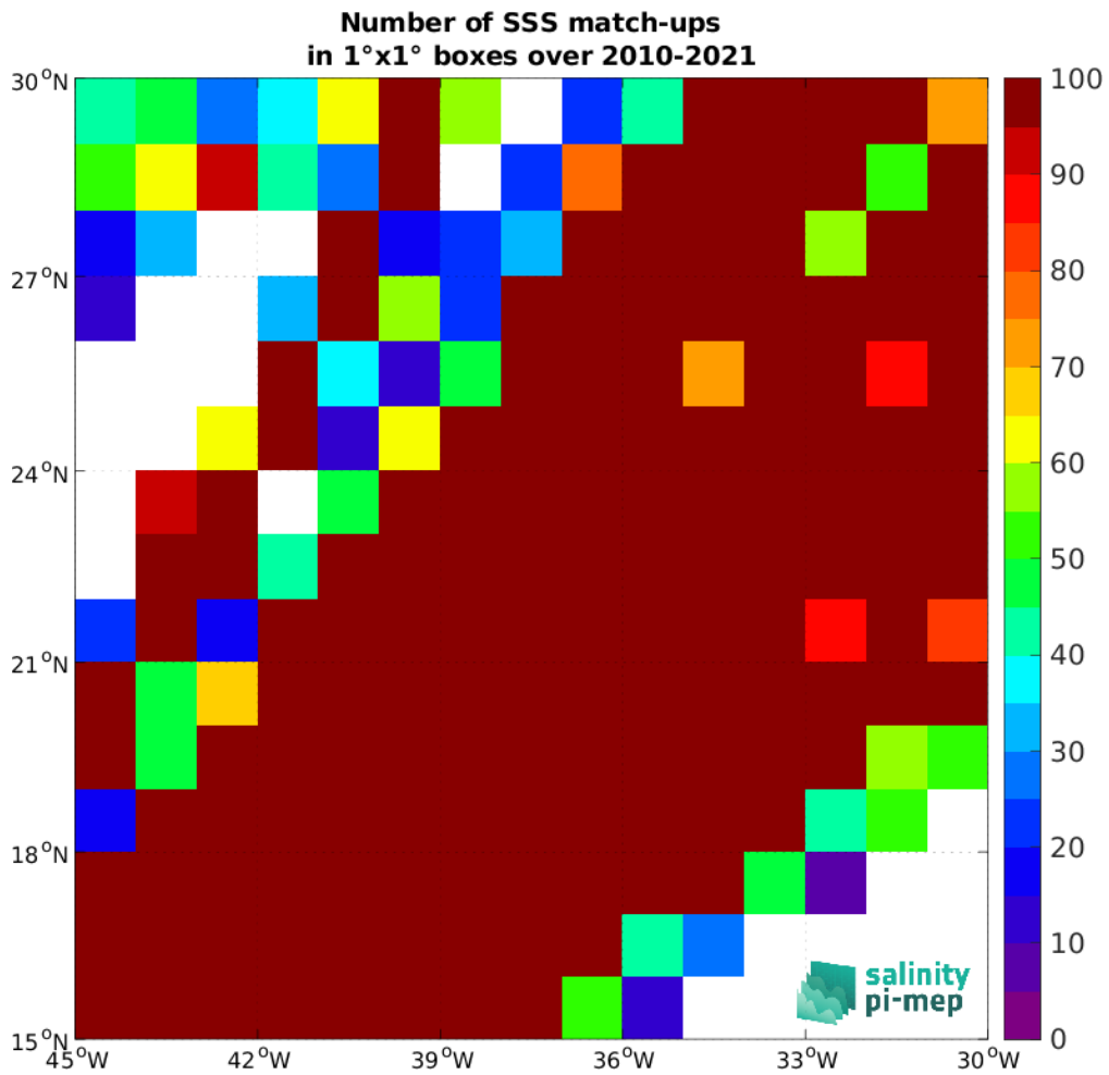
Figure 4: Number of SSS match-ups between TSG (LEGOS-DM) SSS and the SMOS SSS L3 v332 - 9 Days (CATDS-CPDC) SSS product for the SPURS 1 Pi-MEP region over 1°x1° boxes and for the full satellite product period.
