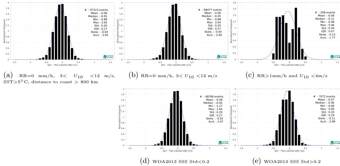
Figure 13: Normalized histogram of \Delta SSS (SMOS SSS L3 v332 - 9 Days (CATDS-CPDC) - TSG (LEGOS-DM)) for 5 different subdatasets corresponding to: RR=0 mm/h, 3 < U_{10} < 12 m/s, SST>5°C, distance to coast > 800 km (a), RR=0 mm/h, 3 < U_{10} < 12 m/s (b), RR>1mm/h and U_{10} < 4 m/s (c), WOA2013 SSS Std<0.2 (d), WOA2013 SSS Std>0.2 (e).
