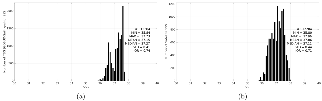
Figure 3: Histograms of SSS from TSG (GOSUD-Sailing-ship) (a) and SMOS SSS L3 v332 - 9 Days (CATDS-CPDC) (b) considering all match-up pairs per bins of 0.1 over the SPURS 1 Pi-MEP region and for the full satellite product period.
