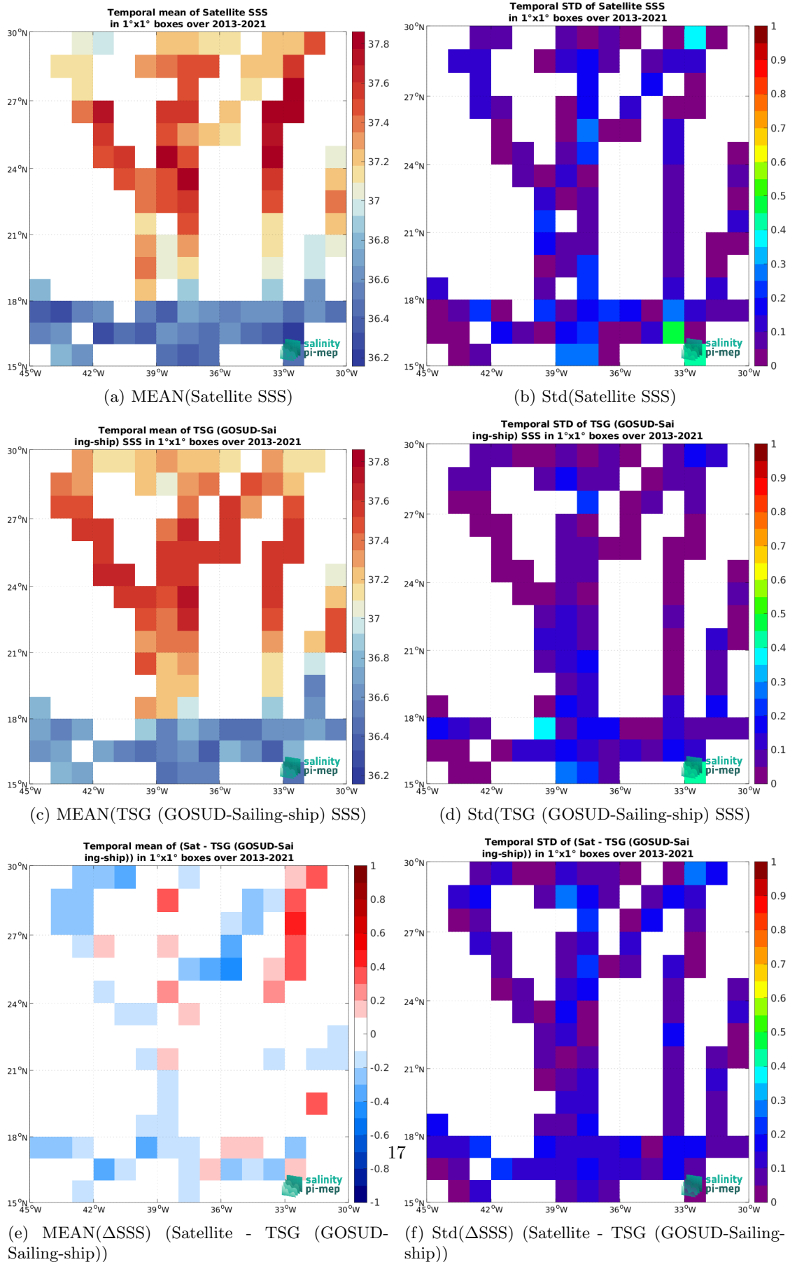
Figure 7: Temporal mean (left) and Std (right) of SSS from SMOS SSS L3 v332 - 9 Days (CATDS-CPDC) (top), TSG (GOSUD-Sailing-ship) (middle), and of \Delta SSS (Satellite - TSG (GOSUD-Sailing-ship)). Only match-up pairs are used to generate these maps.
