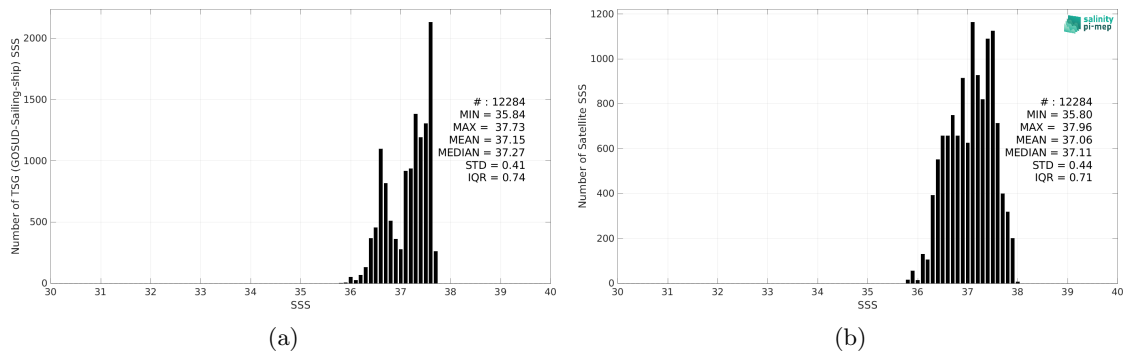
Figure 2: Histograms of SSS from TSG (GOSUD-Sailing-ship) (a) and SMOS SSS L3 v332 - 9 Days (CATDS-CPDC) (b) considering all match-up pairs per bins of 0.1 over the SPURS 1 Pi-MEP region and for the full satellite product period.
