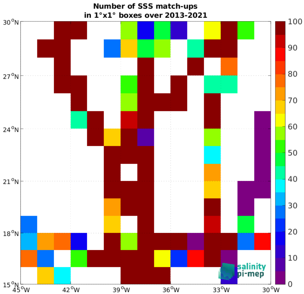
Figure 4: Number of SSS match-ups between TSG (GOSUD-Sailing-ship) SSS and the SMOS SSS L3 v332 - 9 Days (CATDS-CPDC) SSS product for the SPURS 1 Pi-MEP region over 1^\circ \times 1^\circ boxes and for the full satellite product period.
