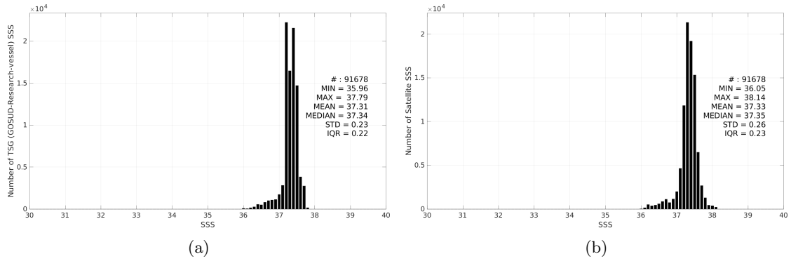
Figure 3: Histograms of SSS from TSG (GOSUD-Research-vessel) (a) and SMOS SSS L3 v332 - 9 Days (CATDS-CPDC) (b) considering all match-up pairs per bins of 0.1 over the SPURS 1 Pi-MEP region and for the full satellite product period.
