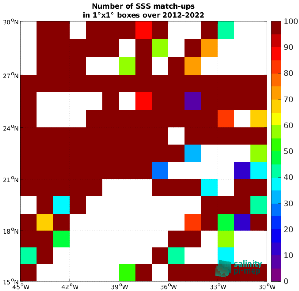
Figure 5: Number of SSS match-ups between TSG (GOSUD-Research-vessel) SSS and the SMOS SSS L3 v332 - 9 Days (CATDS-CPDC) SSS product for the SPURS 1 Pi-MEP region over 1°x1° boxes and for the full satellite product period.
