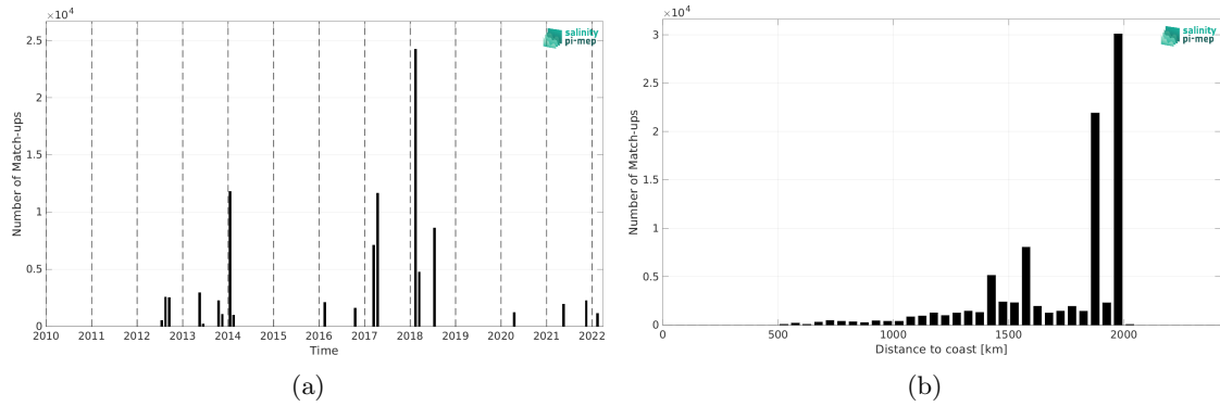
Figure 2: Number of match-ups between TSG (GOSUD-Research-vessel) and SMOS SSS L3 v332 - 9 Days (CATDS-CPDC) SSS as a function of time (a) and as function of the distance to coast (b) over the SPURS 1 Pi-MEP region and for the full satellite product period.
