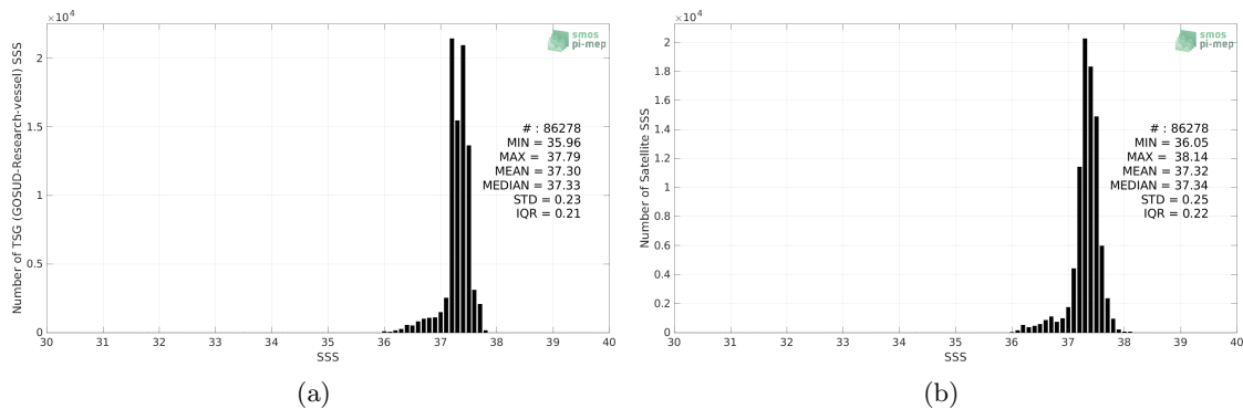
Figure 2: Histograms of SSS from TSG (GOSUD-Research-vessel) (a) and SMOS SSS L3 v332 - 9 Days (CATDS-CPDC) (b) considering all match-up pairs per bins of 0.1 over the SPURS 1 Pi-MEP region and for the full satellite product period.
