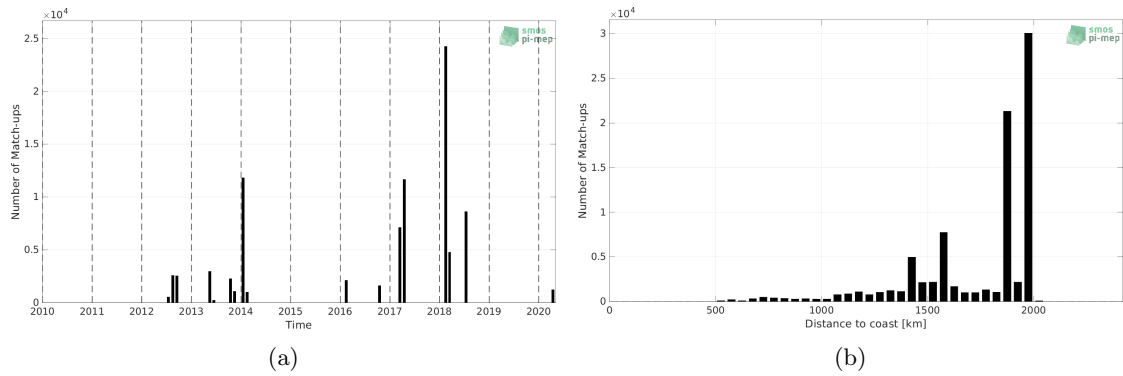
Figure 1: Number of match-ups between TSG (GOSUD-Research-vessel) and SMOS SSS L3 v332 - 9 Days (CATDS-CPDC) SSS as a function of time (a) and as function of the distance to coast (b) over the SPURS 1 Pi-MEP region and for the full satellite product period.
