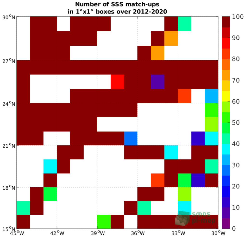
Figure 4: Number of SSS match-ups between TSG (GOSUD-Research-vessel) SSS and the SMOS SSS L3 v332 - 9 Days (CATDS-CPDC) SSS product for the SPURS 1 Pi-MEP region over 1°x1° boxes and for the full satellite product period.
