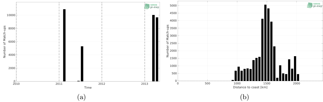
Figure 1: Number of match-ups between TSG (CSIC-UTM) and SMOS SSS L3 v332 - 9 Days (CATDS-CPDC) SSS as a function of time (a) and as function of the distance to coast (b) over the SPURS 1 Pi-MEP region and for the full satellite product period.
