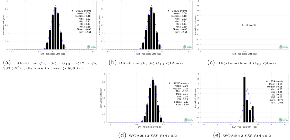
Figure 13: Normalized histogram of \Delta\text{SSS} (SMOS SSS L3 v332 - 9 Days (CATDS-CPDC) - TSG (CSIC-UTM)) for 5 different subdatasets corresponding to: RR=0 mm/h, 3 < U_{10} < 12 m/s, SST >5^{\circ}\text{C} , distance to coast > 800 km (a), RR=0 mm/h, 3 < U_{10} < 12 m/s (b), RR >1 mm/h and U_{10} < 4 m/s (c), WOA2013 SSS Std <0.2 (d), WOA2013 SSS Std >0.2 (e).
