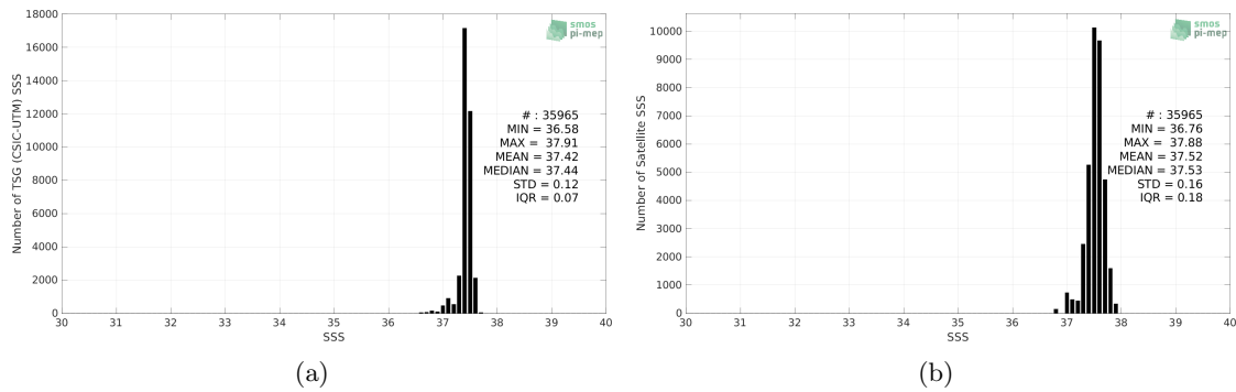
Figure 2: Histograms of SSS from TSG (CSIC-UTM) (a) and SMOS SSS L3 v332 - 9 Days (CATDS-CPDC) (b) considering all match-up pairs per bins of 0.1 over the SPURS 1 Pi-MEP region and for the full satellite product period.
