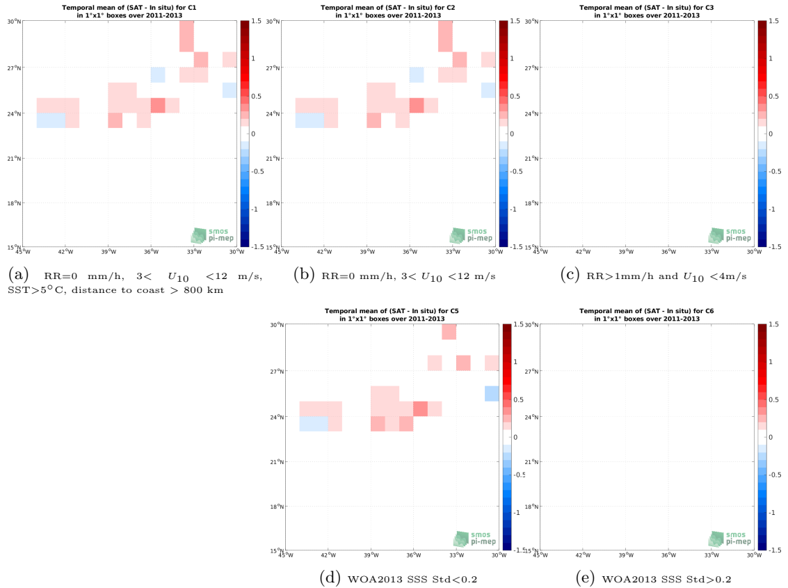
Figure 12: Temporal mean gridded over spatial boxes of size 1^{\circ}\times 1^{\circ} of \Delta\text{SSS} (SMOS SSS L3 v332 - 9 Days (CATDS-CPDC) - TSG (CSIC-UTM)) for 5 different subdatasets corresponding to:RR=0 mm/h, 3 < U_{10} < 12 m/s, SST >5^{\circ}\text{C} , distance to coast > 800 km (a), RR=0 mm/h, 3 < U_{10} < 12 m/s (b), RR >1 mm/h and U_{10} < 4 m/s (c), WOA2013 SSS Std <0.2 (d), WOA2013 SSS Std >0.2 (e).
