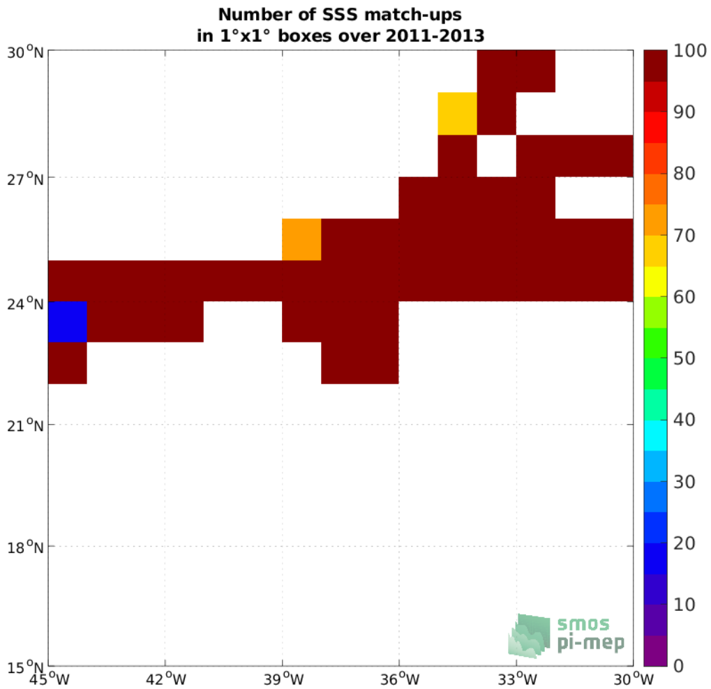
Figure 4: Number of SSS match-ups between TSG (CSIC-UTM) SSS and the SMOS SSS L3 v332 - 9 Days (CATDS-CPDC) SSS product for the SPURS 1 Pi-MEP region over 1°x1° boxes and for the full satellite product period.
