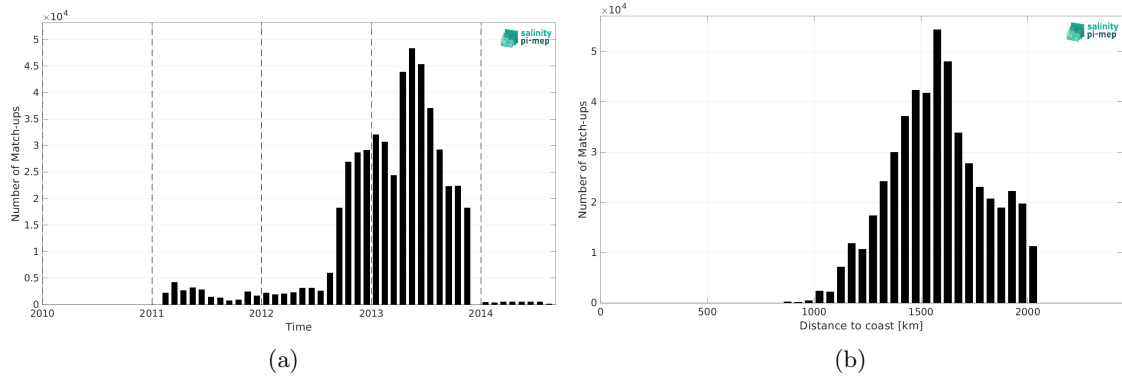
Figure 2: Number of match-ups between Surface drifters and SMOS SSS L3 v332 - 9 Days (CATDS-CPDC) SSS as a function of time (a) and as function of the distance to coast (b) over the SPURS 1 Pi-MEP region and for the full satellite product period.
