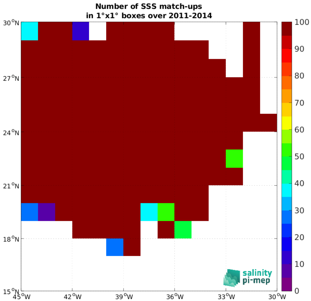
Figure 4: Number of SSS match-ups between Surface drifters SSS and the SMOS SSS L3 v332 - 9 Days (CATDS-CPDC) SSS product for the SPURS 1 Pi-MEP region over 1°x1° boxes and for the full satellite product period.
