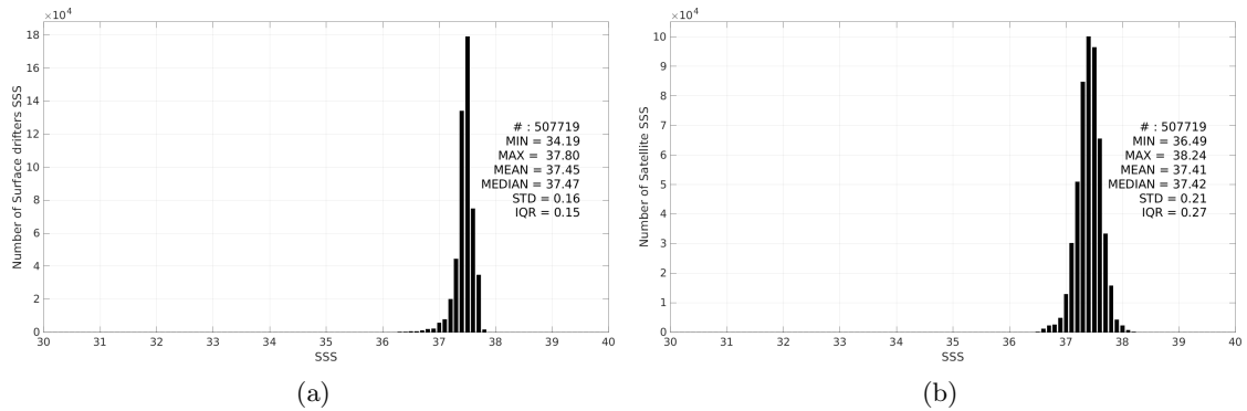
Figure 3: Histograms of SSS from Surface drifters (a) and SMOS SSS L3 v332 - 9 Days (CATDS-CPDC) (b) considering all match-up pairs per bins of 0.1 over the SPURS 1 Pi-MEP region and for the full satellite product period.
