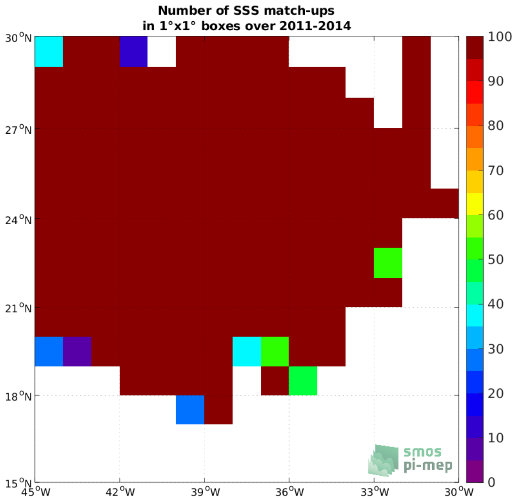
Figure 3: Number of SSS match-ups between Surface drifters SSS and the SMOS SSS L3 v332 - 9 Days (CATDS-CPDC) SSS product for the SPURS 1 Pi-MEP region over 1°x1° boxes and for the full satellite product period.
