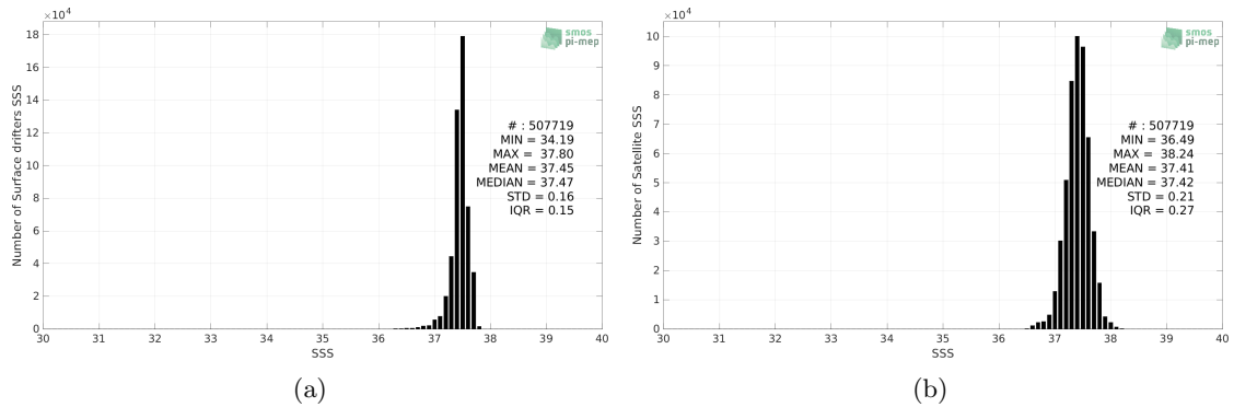
Figure 2: Histograms of SSS from Surface drifters (a) and SMOS SSS L3 v332 - 9 Days (CATDS-CPDC) (b) considering all match-up pairs per bins of 0.1 over the SPURS 1 Pi-MEP region and for the full satellite product period.
