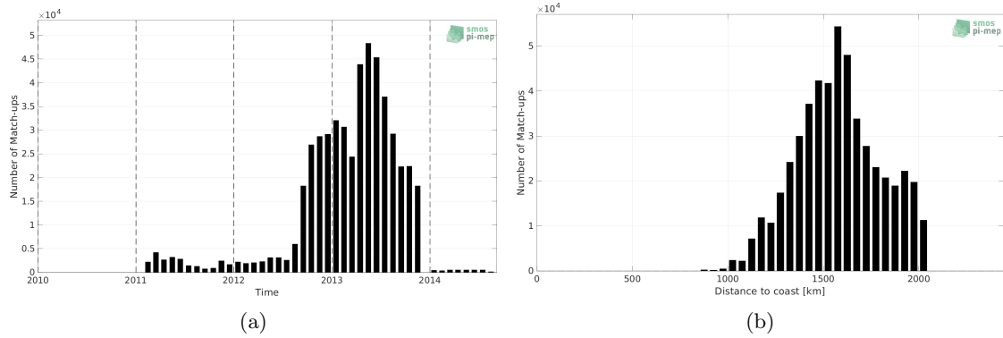
Figure 1: Number of match-ups between Surface drifters and SMOS SSS L3 v332 - 9 Days (CATDS-CPDC) SSS as a function of time (a) and as function of the distance to coast (b) over the SPURS 1 Pi-MEP region and for the full satellite product period.
