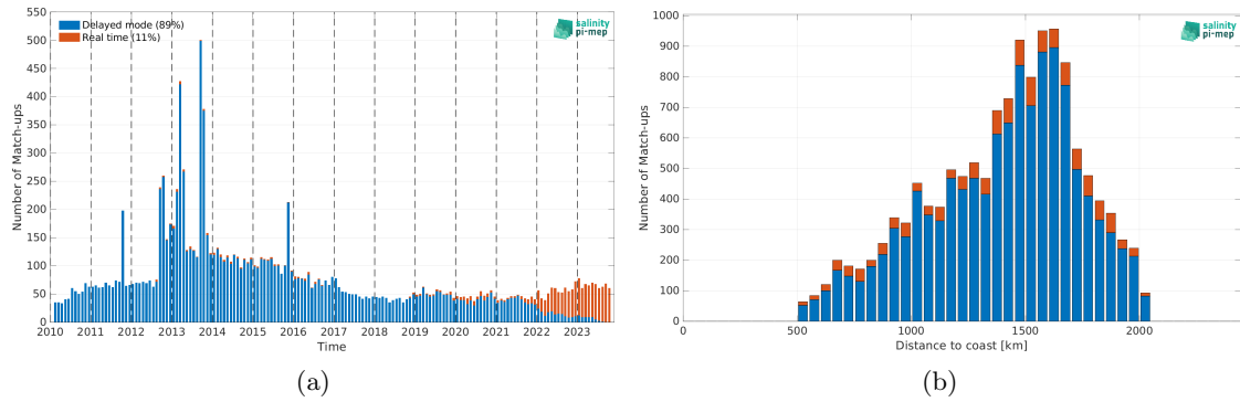
Figure 1: Number of match-ups between Argo and SMOS SSS L3 v332 - 9 Days (CATDS-CPDC) SSS as a function of time (a) and as function of the distance to coast (b) over the SPURS 1 Pi-MEP region and for the full satellite product period.
