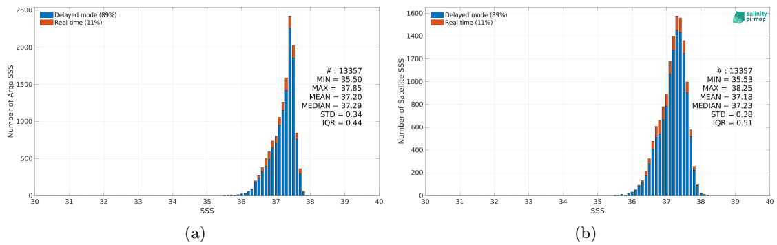
Figure 2: Histograms of SSS from Argo (a) and SMOS SSS L3 v332 - 9 Days (CATDS-CPDC) (b) considering all match-up pairs per bins of 0.1 over the SPURS 1 Pi-MEP region and for the full satellite product period.
