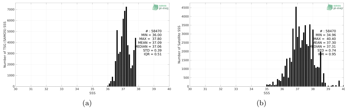
Figure 2: Histograms of SSS from TSG (SAMOS) (a) and SMOS SSS L2Q v331 - 0.25 Deg (CATDS-CPDC) (b) considering all match-up pairs per bins of 0.1 over the SPURS 1 Pi-MEP region and for the full satellite product period.
