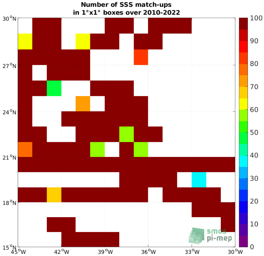
Figure 4: Number of SSS match-ups between TSG (SAMOS) SSS and the SMOS SSS L2Q v331 - 0.25 Deg (CATDS-CPDC) SSS product for the SPURS 1 Pi-MEP region over 1°x1° boxes and for the full satellite product period.
