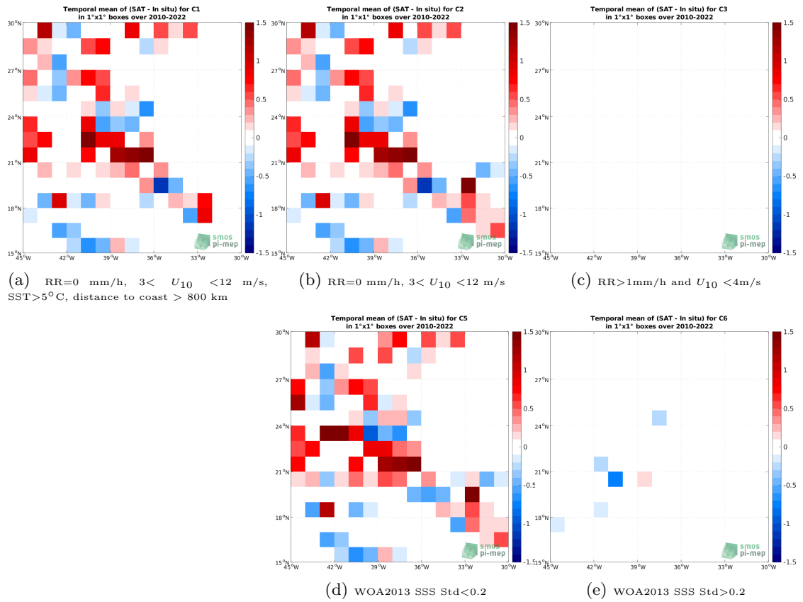
Figure 12: Temporal mean gridded over spatial boxes of size 1^\circ \times 1^\circ of \Delta SSS (SMOS SSS L2Q v331 - 0.25 Deg (CATDS-CPDC) - TSG (SAMOS)) for 5 different subdatasets corresponding to:RR=0 mm/h, 3 < U_{10} < 12 m/s, SST >5^\circ C, distance to coast > 800 km (a), RR=0 mm/h, 3 < U_{10} < 12 m/s (b), RR >1 mm/h and U_{10} < 4 m/s (c), WOA2013 SSS Std <0.2 (d), WOA2013 SSS Std >0.2 (e).
