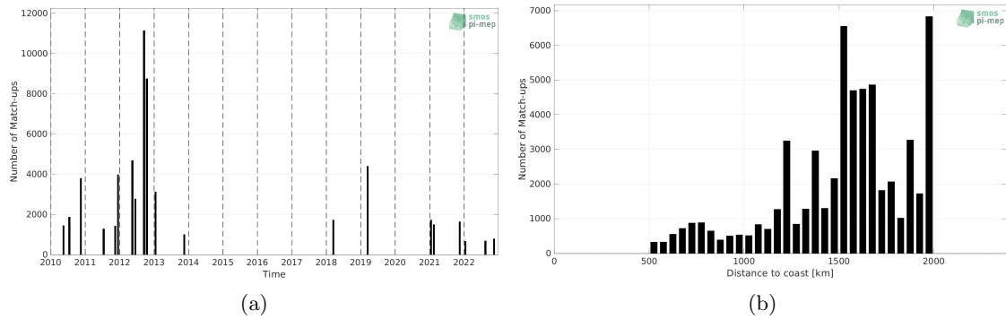
Figure 1: Number of match-ups between TSG (SAMOS) and SMOS SSS L2Q v331 - 0.25 Deg (CATDS-CPDC) SSS as a function of time (a) and as function of the distance to coast (b) over the SPURS 1 Pi-MEP region and for the full satellite product period.
