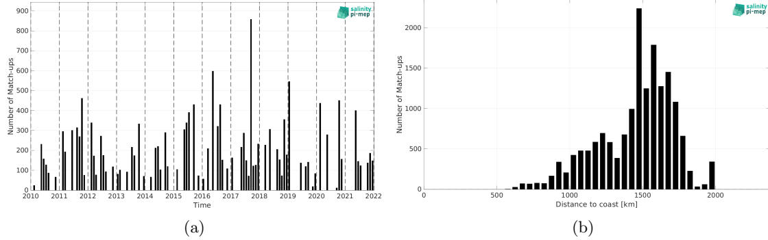
Figure 1: Number of match-ups between TSG (LEGOS-DM) and SMOS SSS L2Q v331 - 0.25 Deg (CATDS-CPDC) SSS as a function of time (a) and as function of the distance to coast (b) over the SPURS 1 Pi-MEP region and for the full satellite product period.
