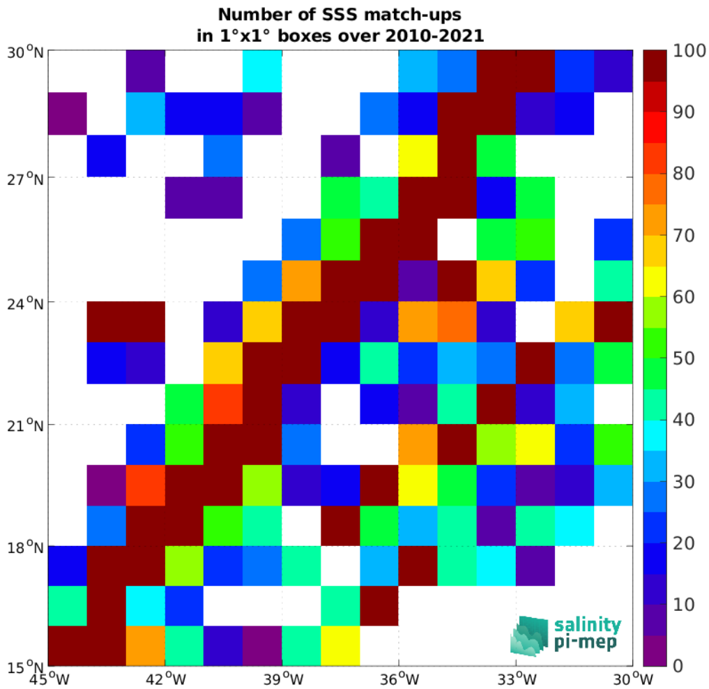
Figure 4: Number of SSS match-ups between TSG (LEGOS-DM) SSS and the SMOS SSS L2Q v331 - 0.25 Deg (CATDS-CPDC) SSS product for the SPURS 1 Pi-MEP region over 1°x1° boxes and for the full satellite product period.
