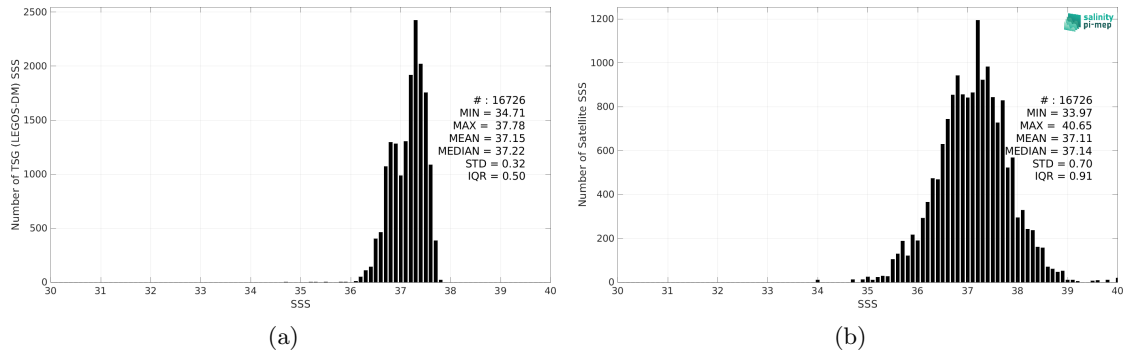
Figure 2: Histograms of SSS from TSG (LEGOS-DM) (a) and SMOS SSS L2Q v331 - 0.25 Deg (CATDS-CPDC) (b) considering all match-up pairs per bins of 0.1 over the SPURS 1 Pi-MEP region and for the full satellite product period.
