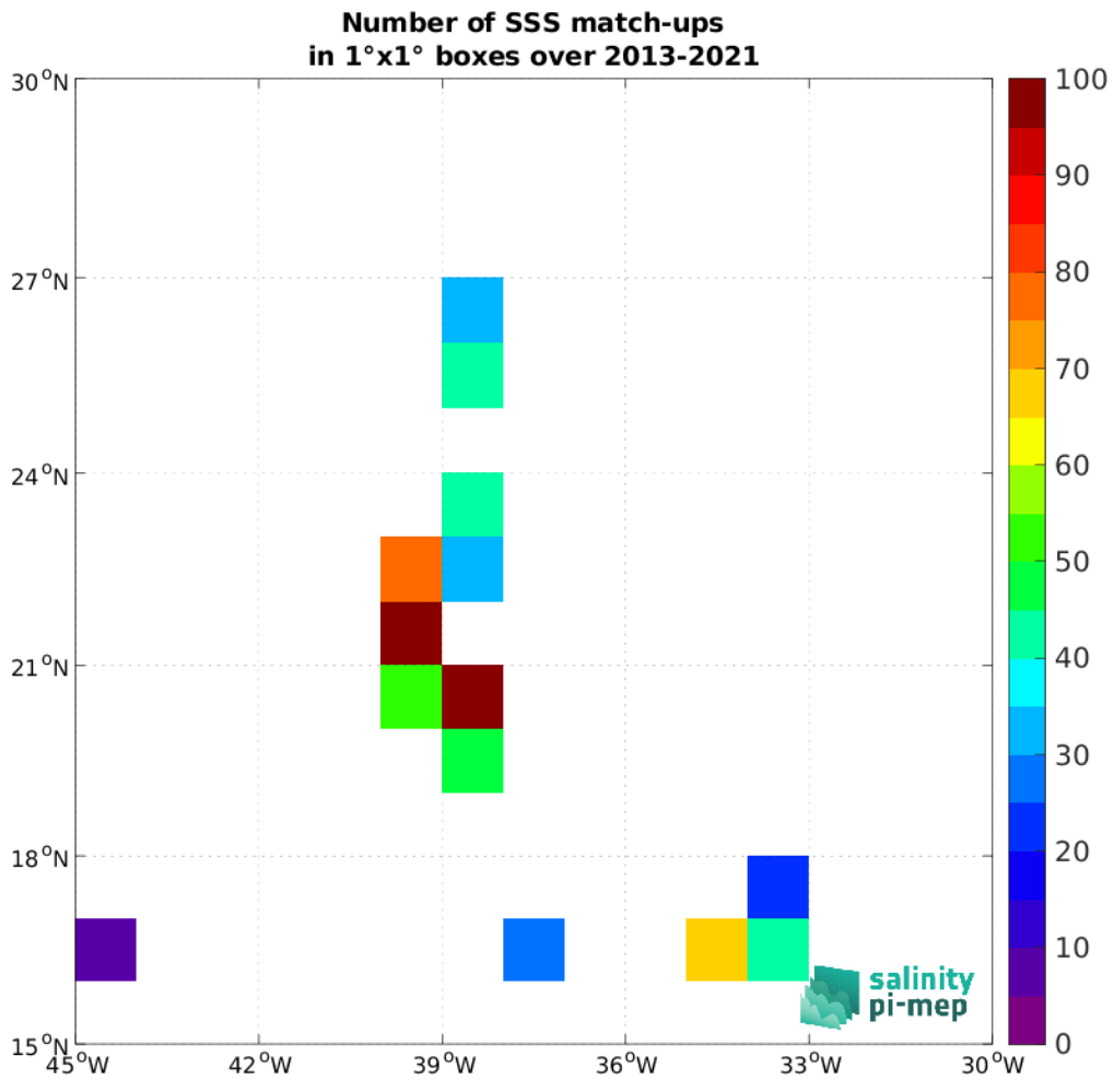
Figure 4: Number of SSS match-ups between TSG (GOSUD-Sailing-ship) SSS and the SMOS SSS L2Q v331 - 0.25 Deg (CATDS-CPDC) SSS product for the SPURS 1 Pi-MEP region over 1^\circ \times 1^\circ boxes and for the full satellite product period.
