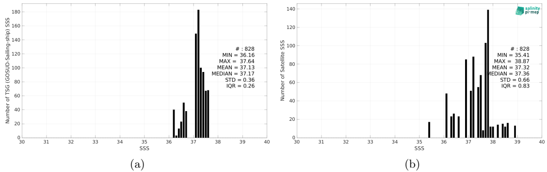
Figure 2: Histograms of SSS from TSG (GOSUD-Sailing-ship) (a) and SMOS SSS L2Q v331 - 0.25 Deg (CATDS-CPDC) (b) considering all match-up pairs per bins of 0.1 over the SPURS 1 Pi-MEP region and for the full satellite product period.
