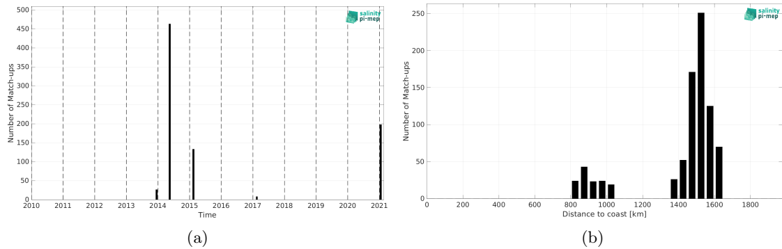
Figure 1: Number of match-ups between TSG (GOSUD-Sailing-ship) and SMOS SSS L2Q v331 - 0.25 Deg (CATDS-CPDC) SSS as a function of time (a) and as function of the distance to coast (b) over the SPURS 1 Pi-MEP region and for the full satellite product period.
