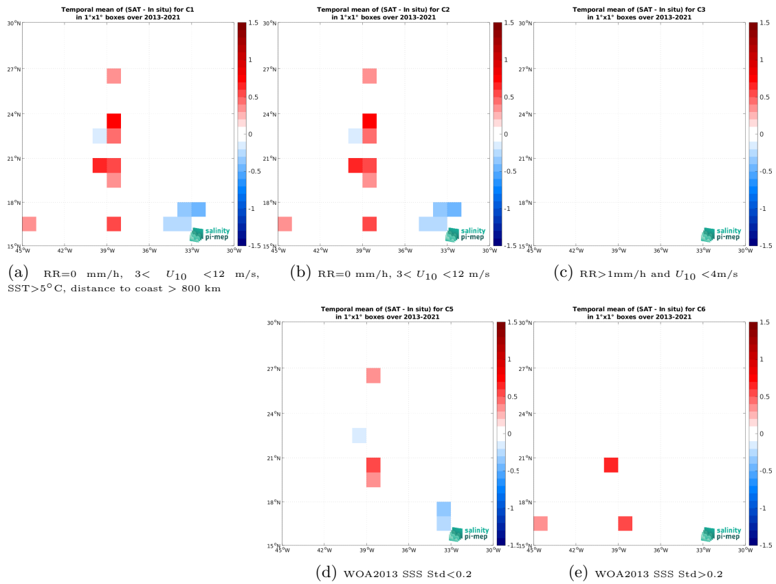
Figure 12: Temporal mean gridded over spatial boxes of size 1^\circ \times 1^\circ of \Delta SSS (SMOS SSS L2Q v331 - 0.25 Deg (CATDS-CPDC) - TSG (GOSUD-Sailing-ship)) for 5 different subdatasets corresponding to: RR=0 mm/h, 3 < U_{10} < 12 m/s, SST > 5°C, distance to coast > 800 km (a), RR=0 mm/h, 3 < U_{10} < 12 m/s (b), RR > 1mm/h and U_{10} < 4 m/s (c), WOA2013 SSS Std < 0.2 (d), WOA2013 SSS Std > 0.2 (e).
