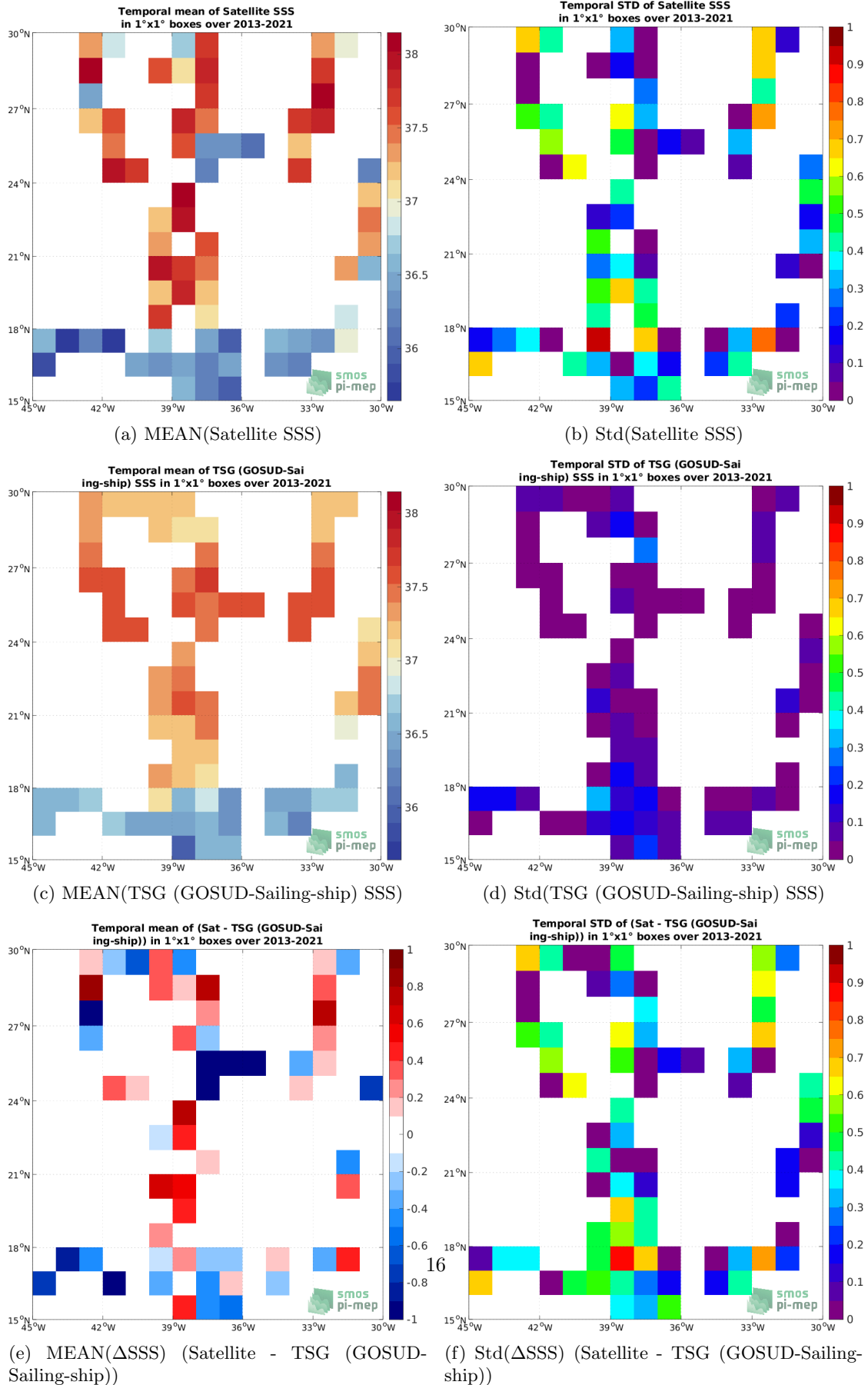
Figure 6: Temporal mean (left) and Std (right) of SSS from SMOS SSS L2Q v331 - 0.25 Deg (CATDS-CPDC) (top), TSG (GOSUD-Sailing-ship) (middle), and of \Delta SSS (Satellite - TSG (GOSUD-Sailing-ship)). Only match-up pairs are used to generate these maps.
